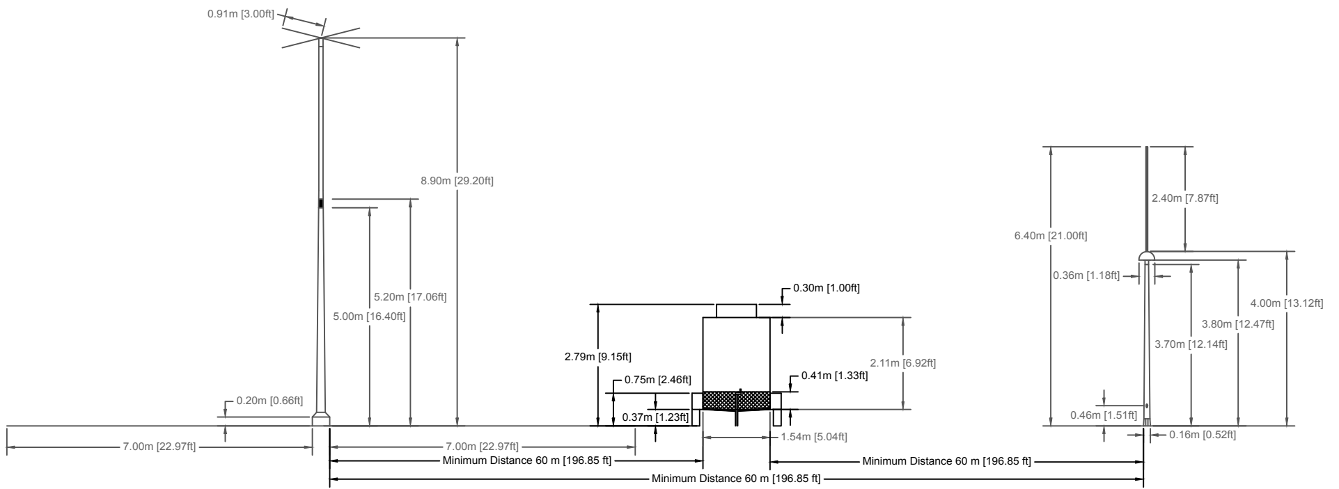
Transmit Antenna
