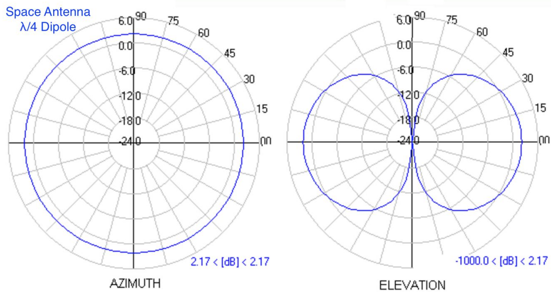
Figure 2: Satellite transmit and receive antenna pattern.
