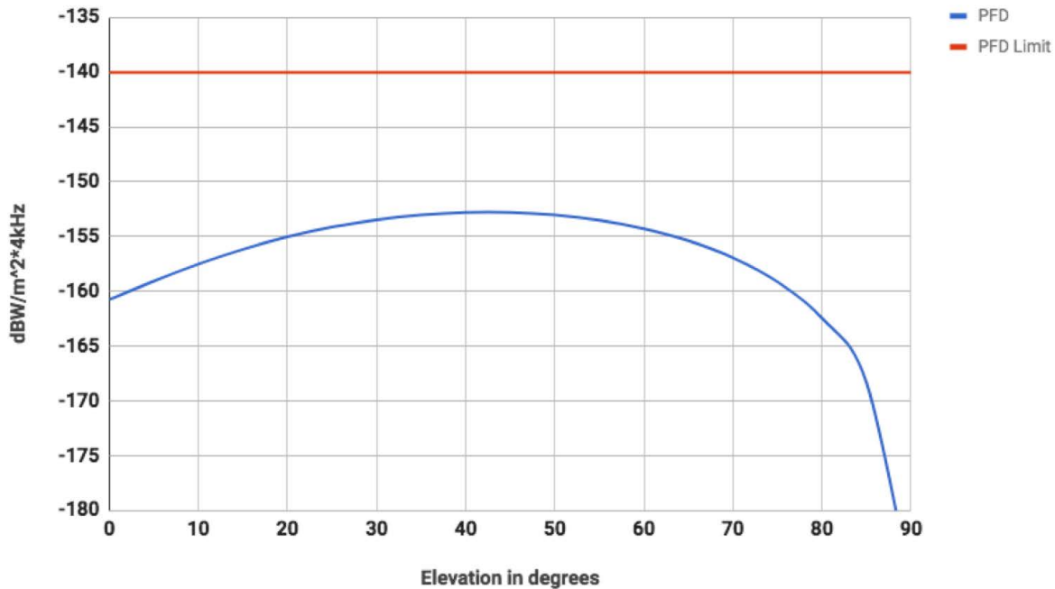
Figure 1. PFD at Earth's surface produced by a satellite transmission
