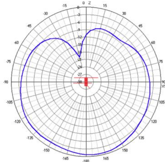
Figure 24 Experimental UHF Satellite Transmit/Receive Antenna Radiation Pattern
