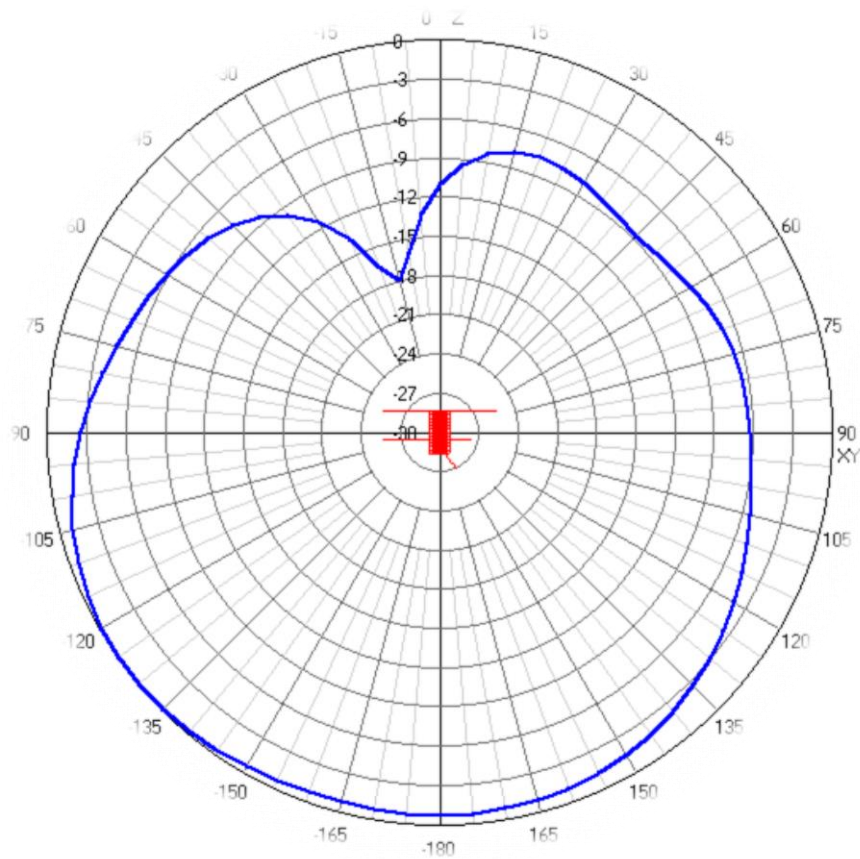
UTX/URX - UHF Satellite Transmit/Receive Radiation Pattern.
