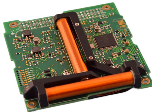
Figure 4. iMTQ Magnetorquer Board.
