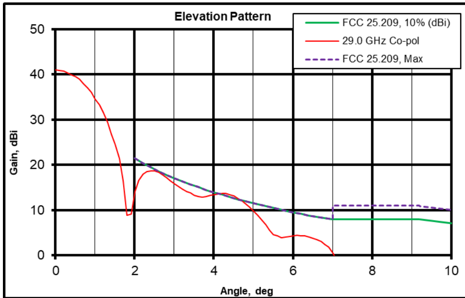
Figure 5. EL Cut, 0° to +10°
