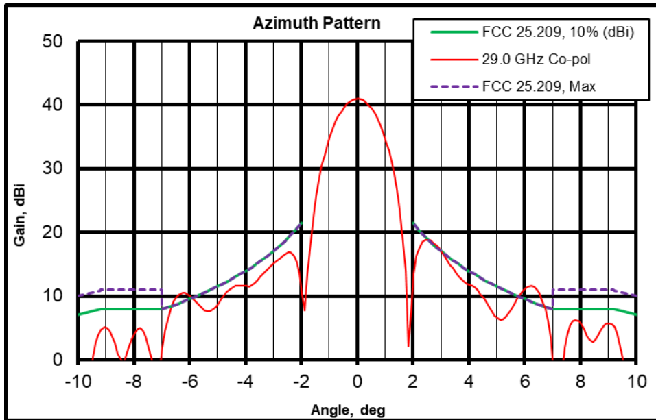
Figure 1. AZ Cut, -10^{\circ} to +10^{\circ}
