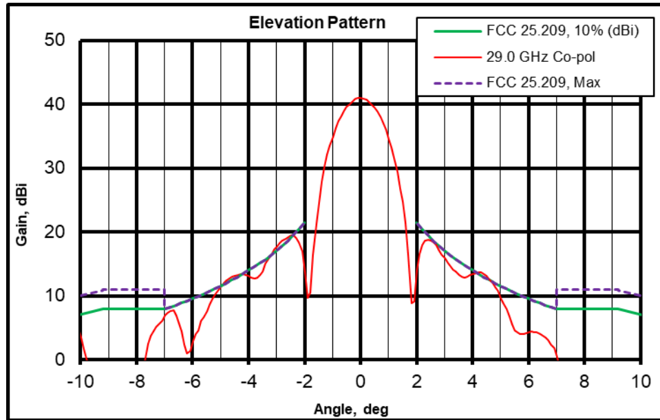
Figure 4. EL Cut, -10^{\circ} to +10^{\circ}
