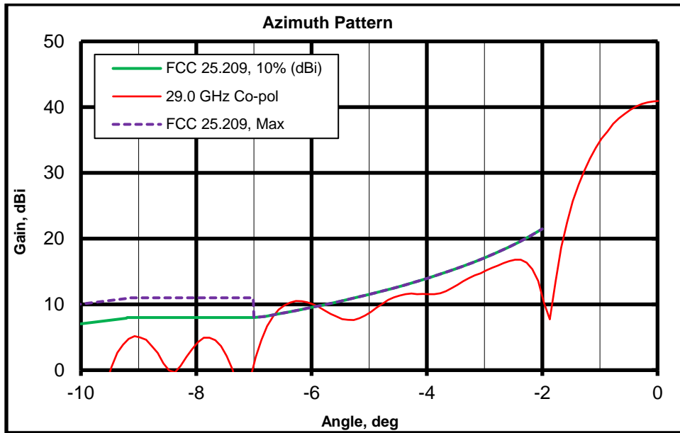
Figure 3. AZ Cut, -10^{\circ} to 0^{\circ}
