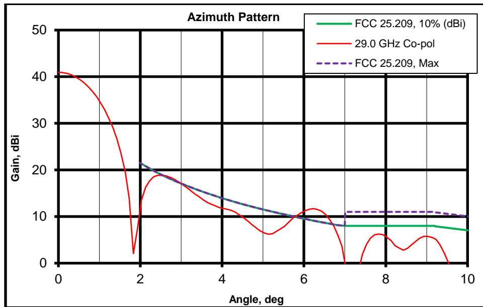
Figure 2. AZ Cut, 0^{\circ} to +10^{\circ}
