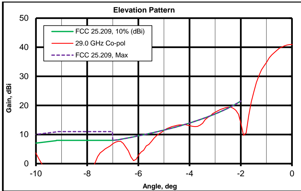
Figure 6. EL Cut, -10° to 0°
