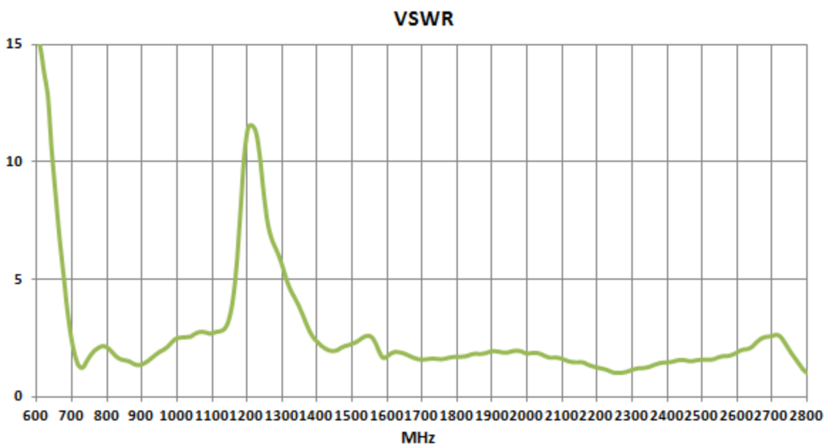
Figure 2. VSWR of FXUB63 Antenna.
