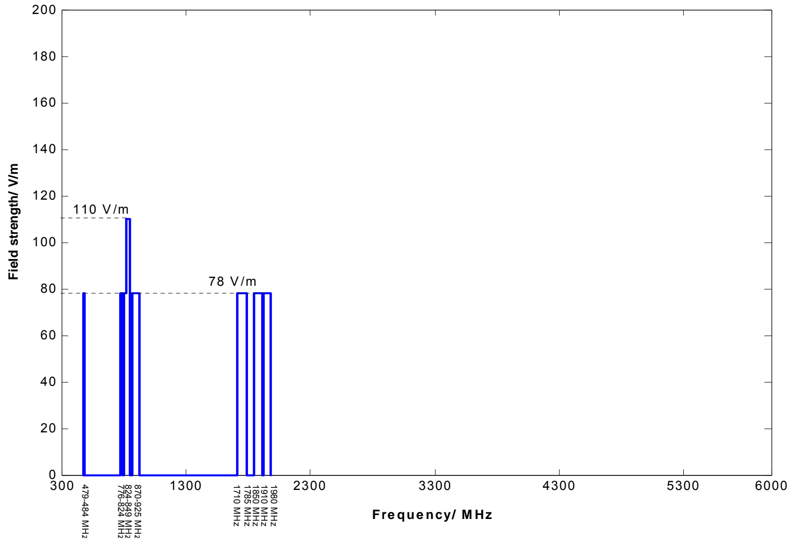
FIGURE 15 : REQUIRED FIELD STRENGTH LEVELS ONTO EUT FOR CW-LIKE T-PED SIGNALS INCLUDING 6DB MARGIN
