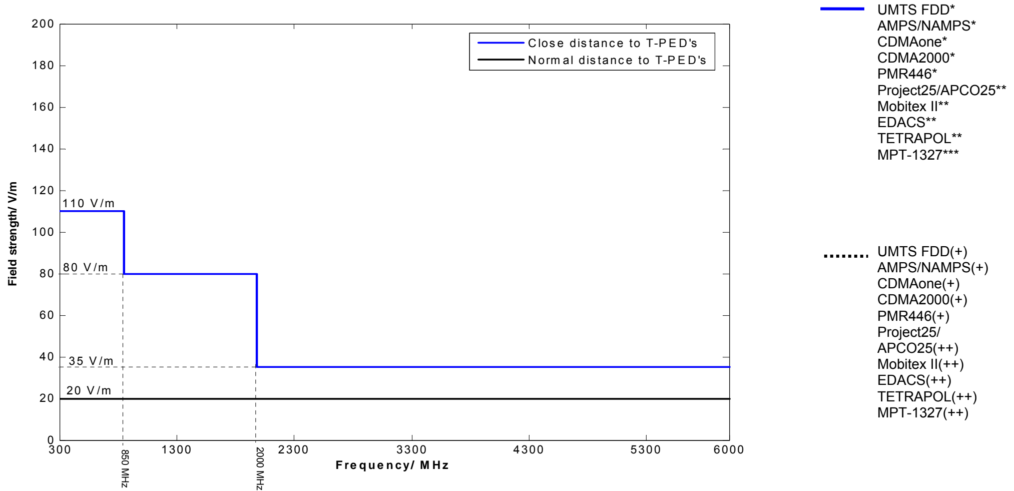
FIGURE 19 : REQUIRED RADIATED FIELD STRENGTH FOR CW-LIKE (FDMA) T-PED SIGNALS INCLUDING 6 DB MARGINS FOR LABORATORY EQUIPMENT QUALIFICATION
