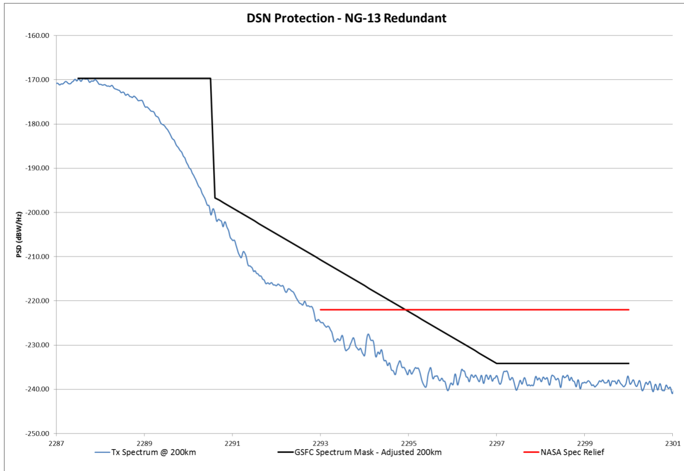
Figure 3 DSN Performance of Emission Designator 6M16G1D with ERP of 4.7 W – Redundant Transmitter
