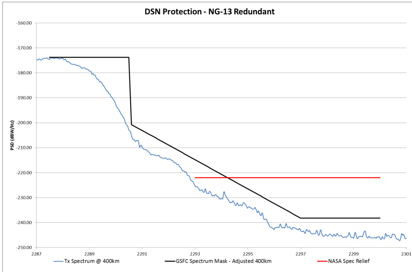
Figure 5 DSN Performance of Emission Designator 6M16G1D with ERP of 7.3 W – Redundant Transmitter
