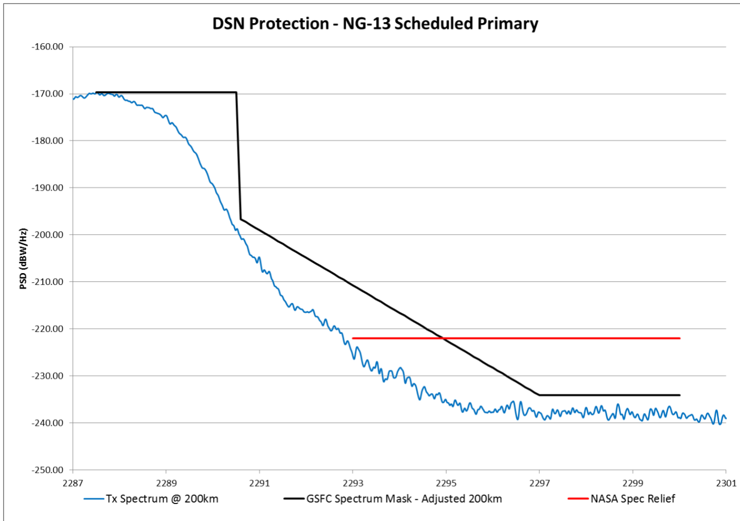
Figure 2 DSN Performance of Emission Designator 6M16G1D with ERP of 4.7 W – Primary Transmitter
