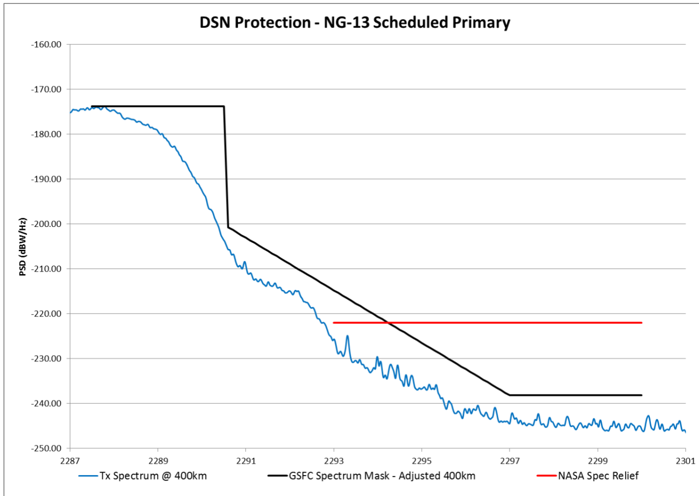
Figure 4 DSN Performance of Emission Designator 6M16G1D with ERP of 7.3 W – Primary Transmitter
