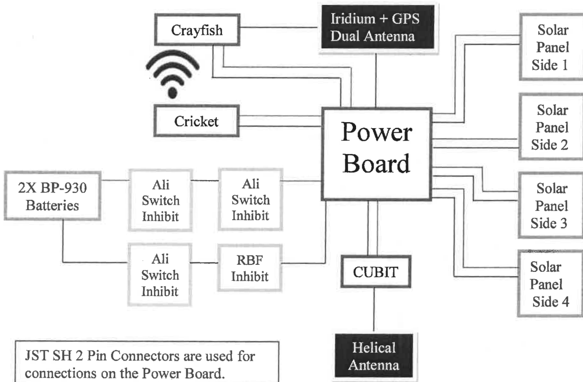
TechEdSat-7 Wiring Diagram
