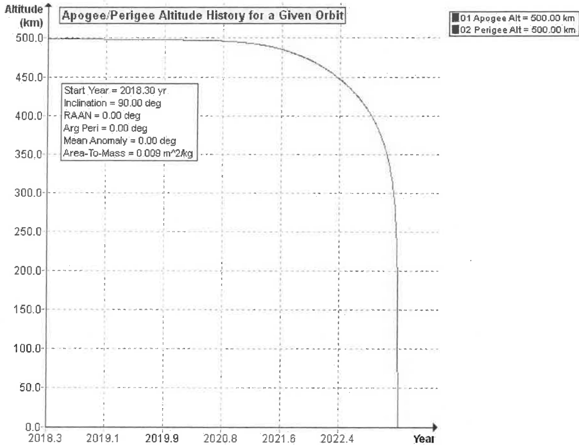
Figure 3: TechEdSat-7 Orbit History for Case 2: Failed Deployment
