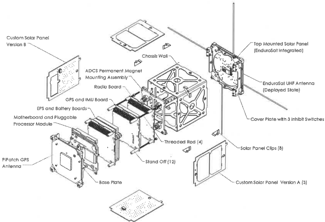
Figure 9: Libertas Expanded View
