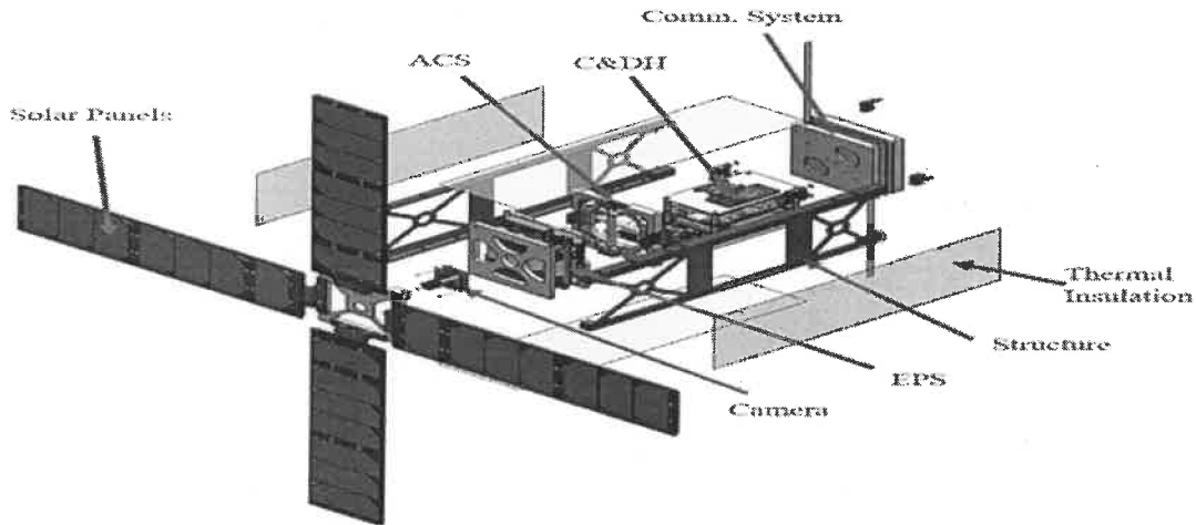
Figure 5: SPACE HAUC Expanded View
