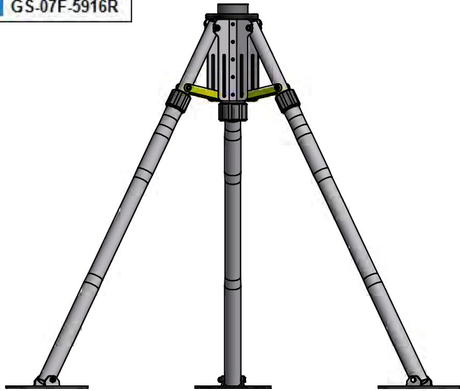
Tripod with Base Plates P/N: BSM2-P-T200-POD-000 14.2 lbs / 6.4 kg
