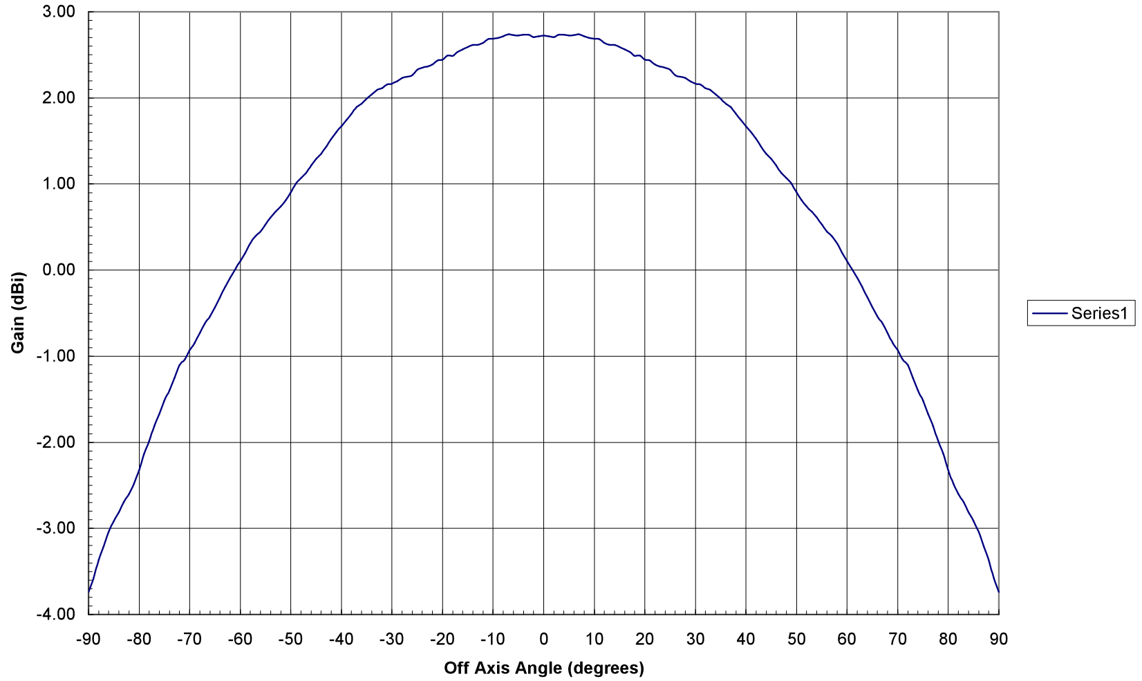
Attachment 20 - User Terminal Co-Polar Radiation Pattern - Transmit
