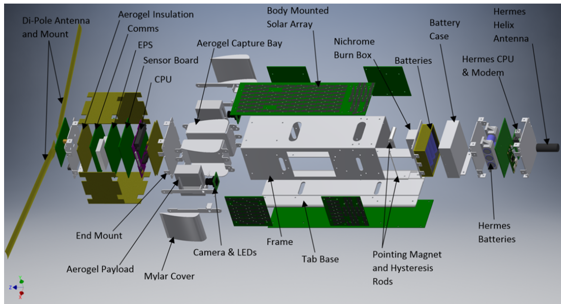
Figure 2: CACTUS-1 Expanded View
