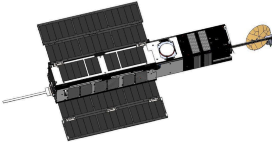
Figure 11: PolarCube Expanded View
