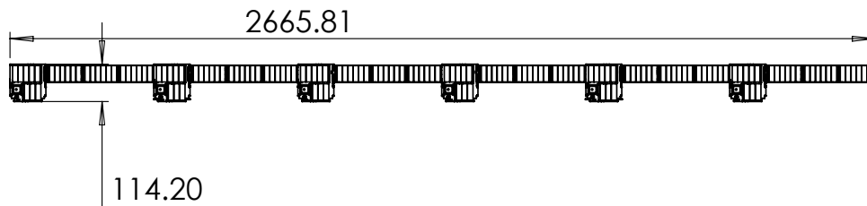
Figure 4 ThinSat 6T Spacecraft, Dimensions in mm
