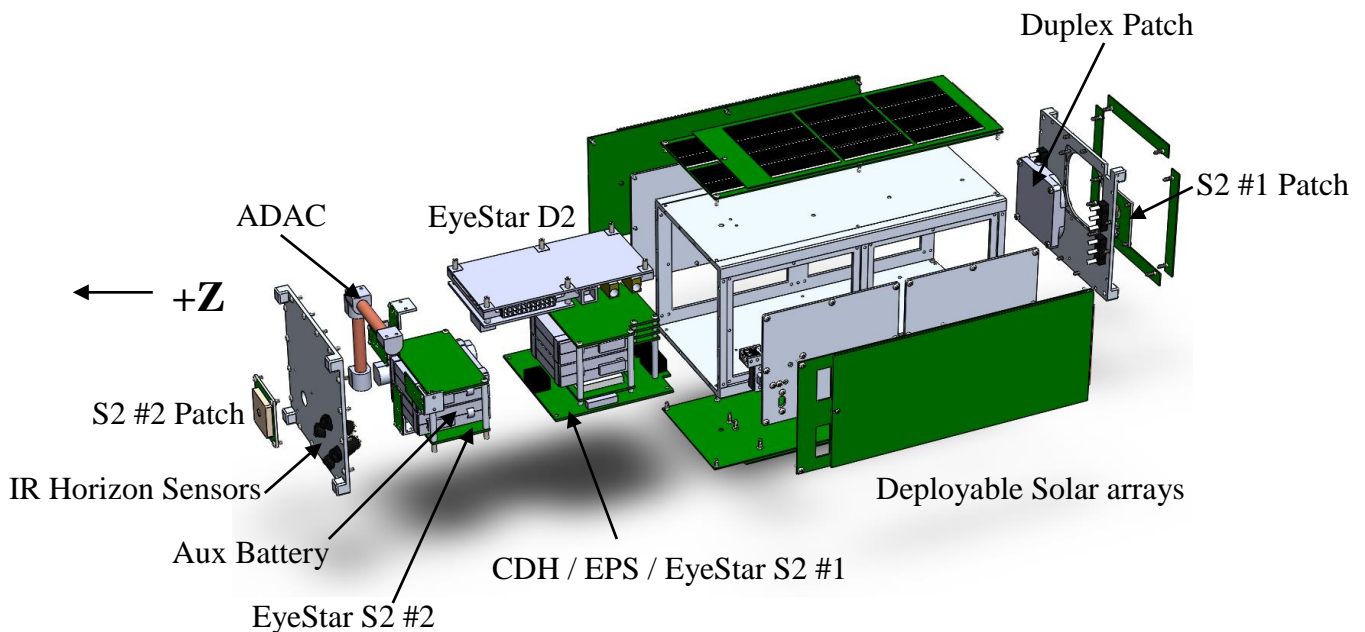
Figure 1 NLSAT-1 Overview
