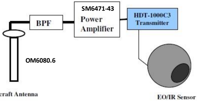
Airborne Equipment
