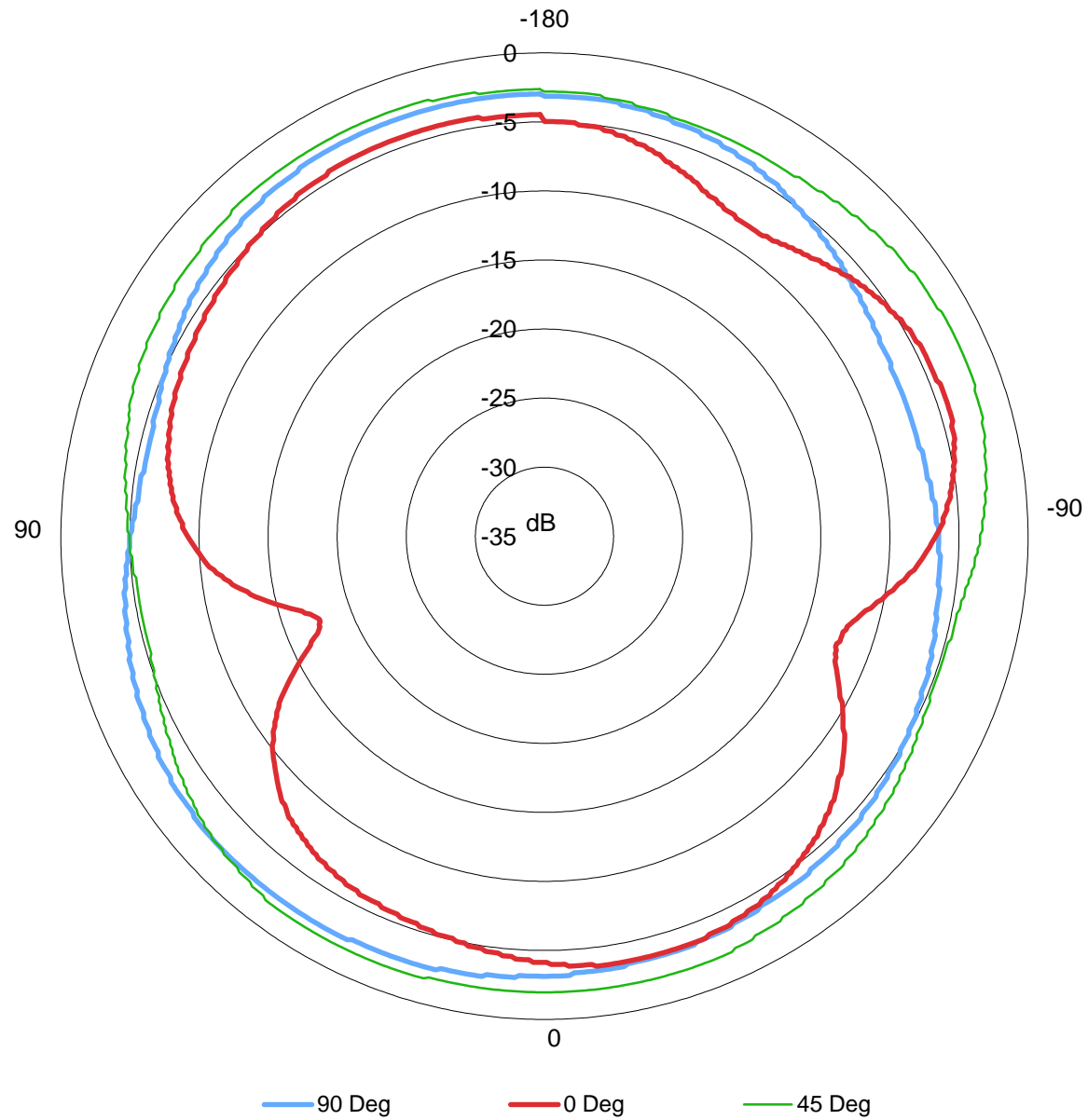
CXBN-2 437 MHz RHCP Antenna Pattern
