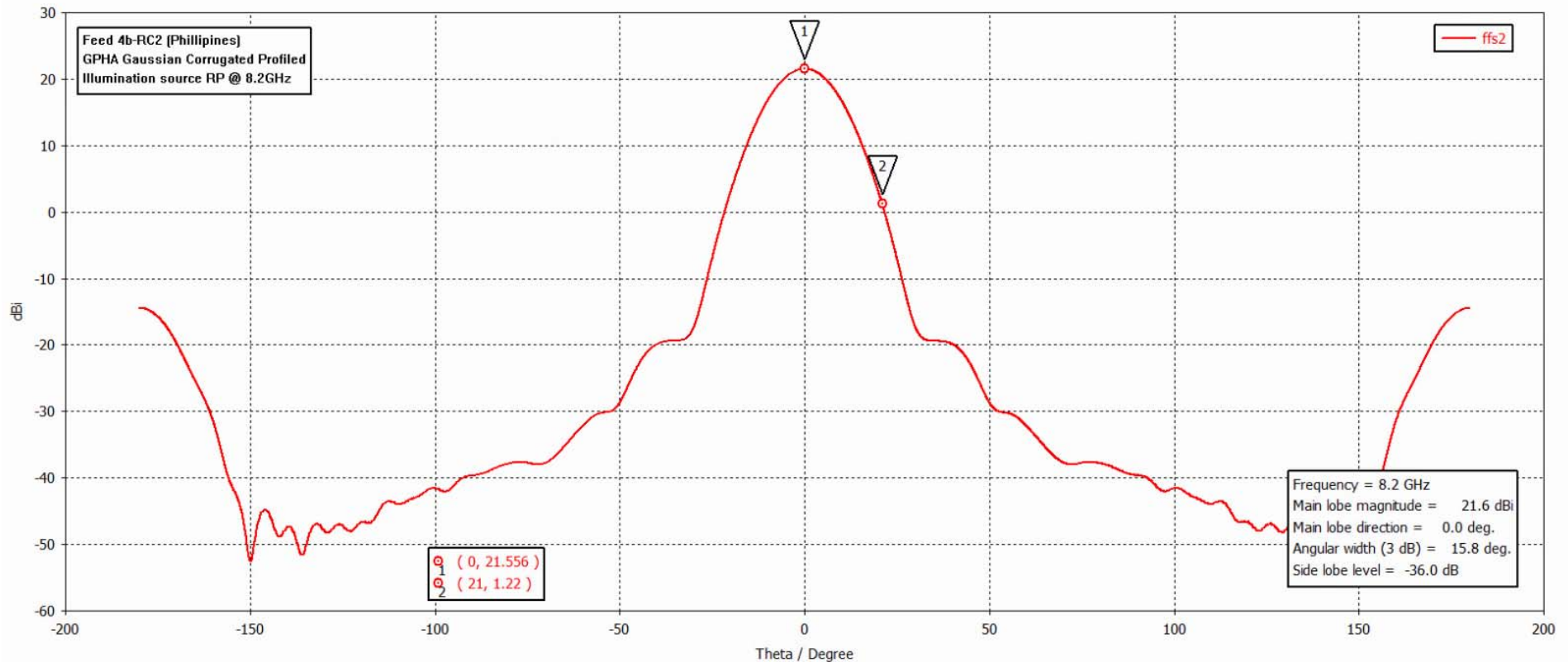
Farfield Source [ffs2] Realized Gain Abs (Phi=90)
