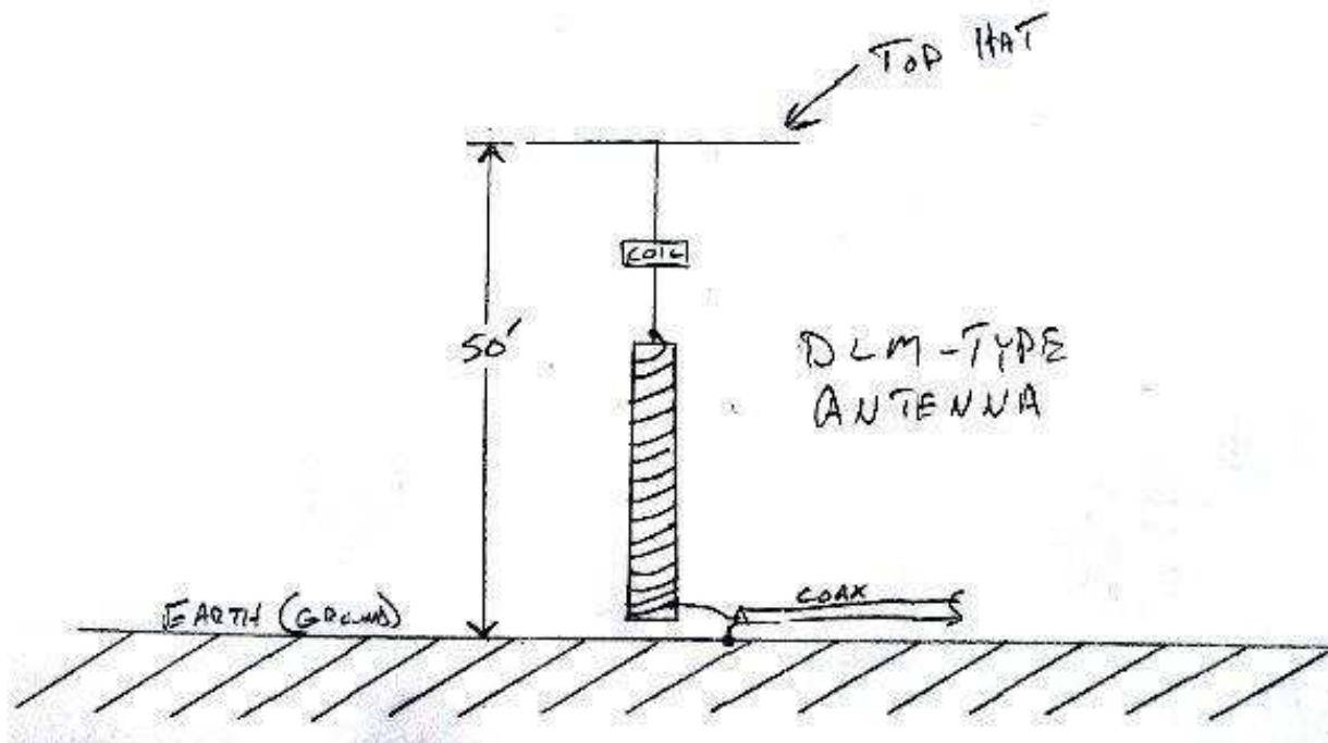
DLM (Distributed Loaded Monopole) Antenna Drawing, Height Detail
