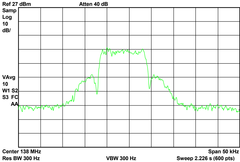
Lithium - 1 GFSK 9600 Baud Output Spectrum
