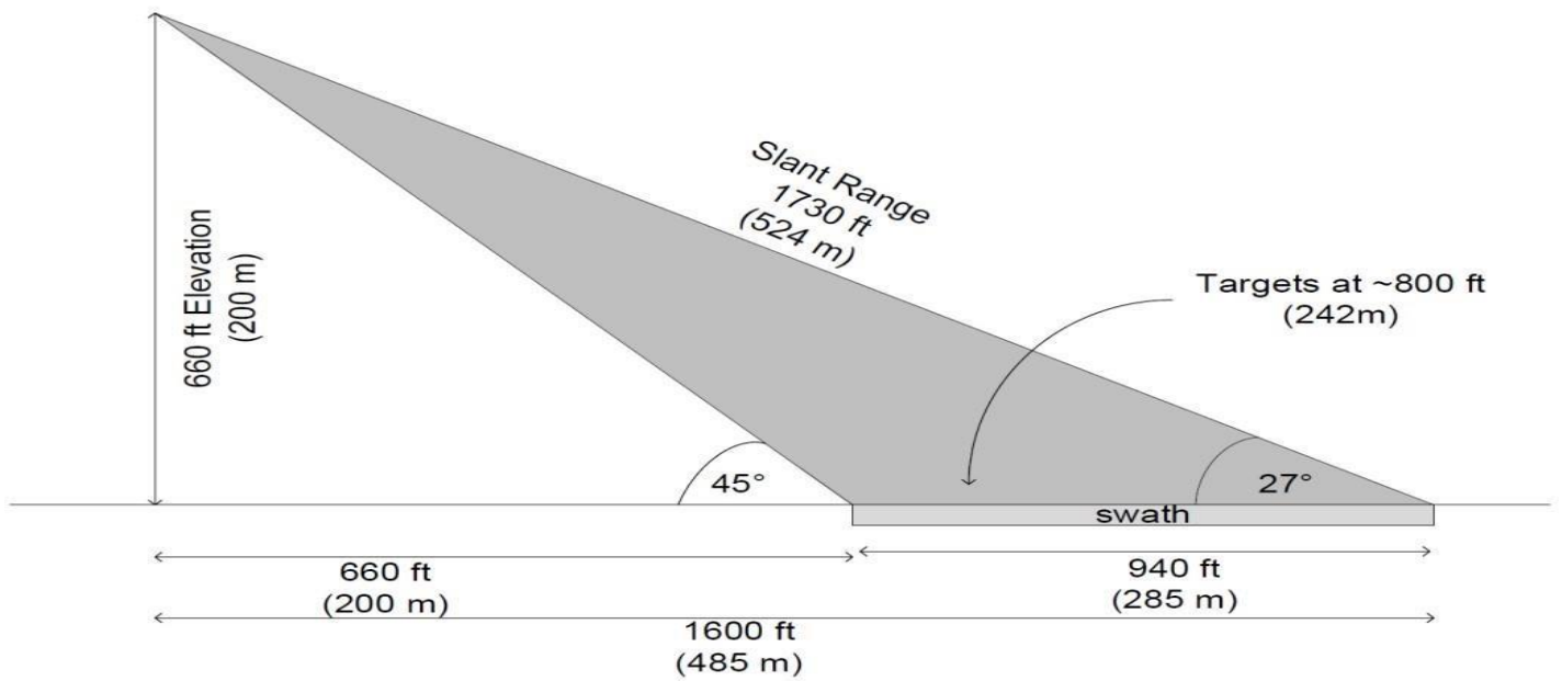
Figure 2. Example SAR geometry, from an airborne platform.
