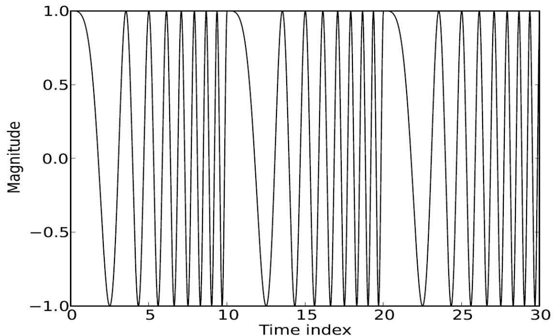
Figure 1. Example LFM chirp signal, increasing in frequency from left to right, then repeating.
