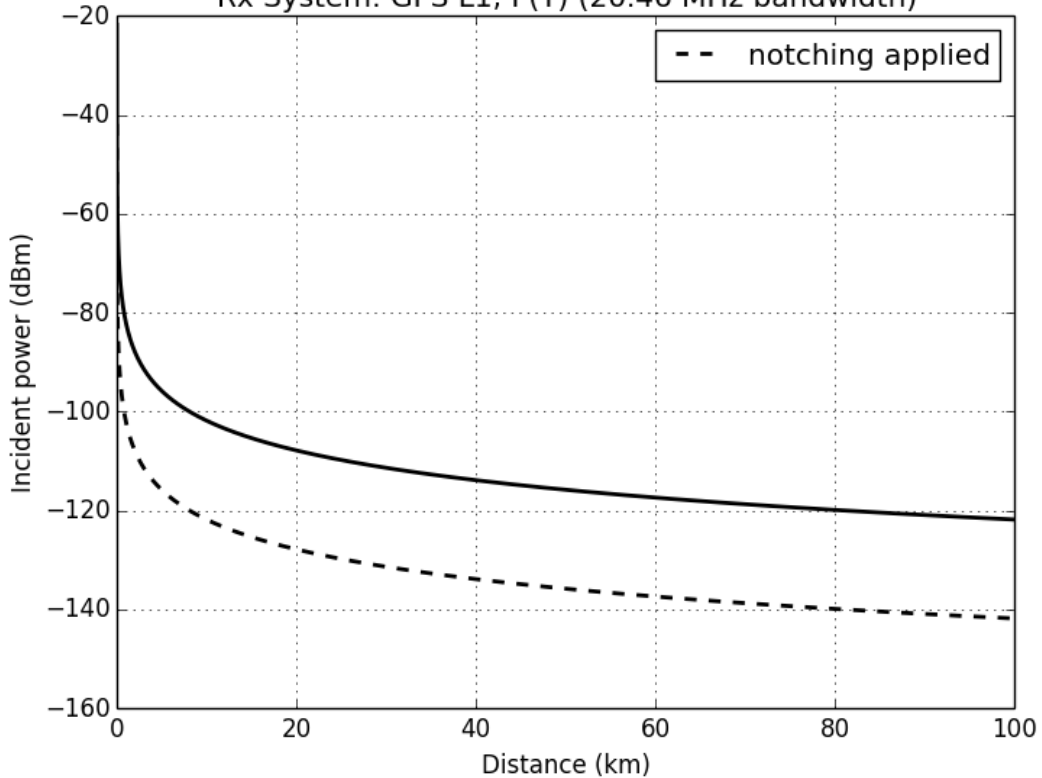
IMSAR UWB SAR electromagnetic compatibility Rx System: GPS L1, P(Y) (20.46 MHz bandwidth)
