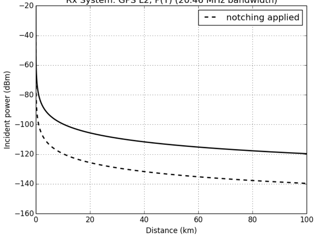
IMSAR UWB SAR electromagnetic compatibility Rx System: GPS L2, P(Y) (20.46 MHz bandwidth)
