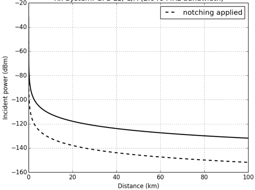
IMSAR UWB SAR electromagnetic compatibility Rx System: GPS L1, C/A (2.046 MHz bandwidth)
