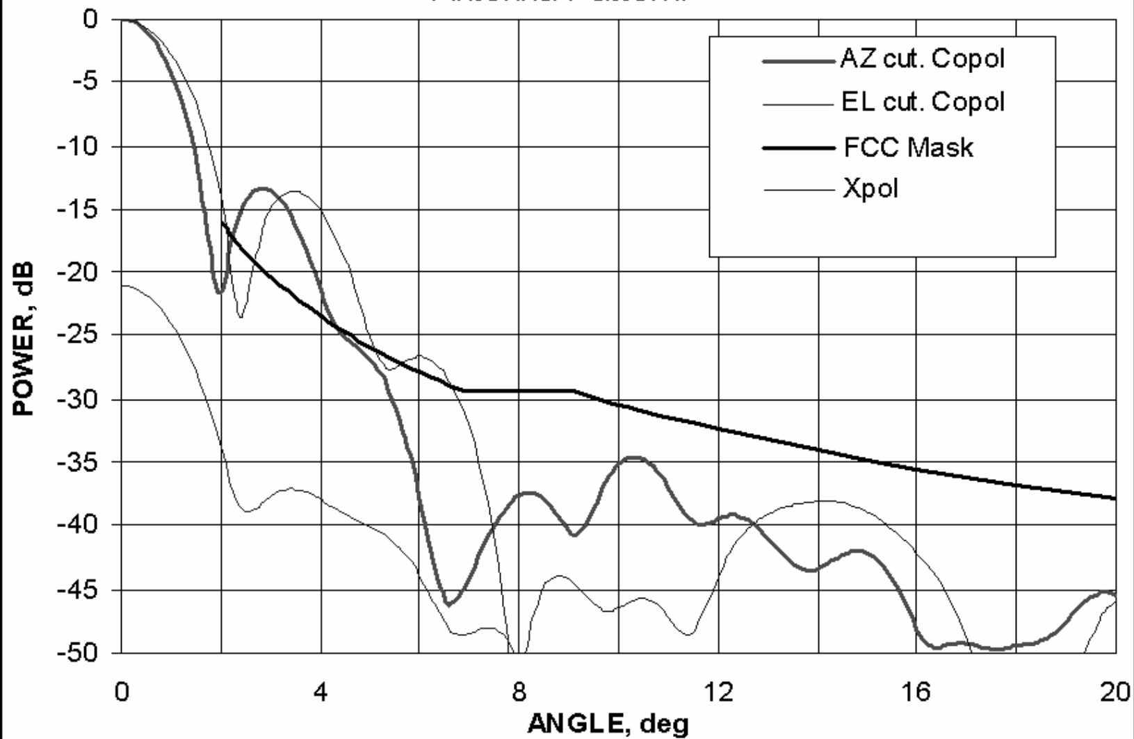
Antenna Pattern.
