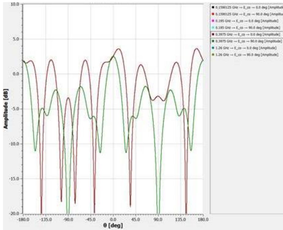
Figure 2-9: BBDA Directivity, 397.5 MHz
