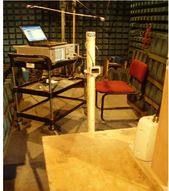
Photo #3. RE investigation setup in anechoic chamber.
