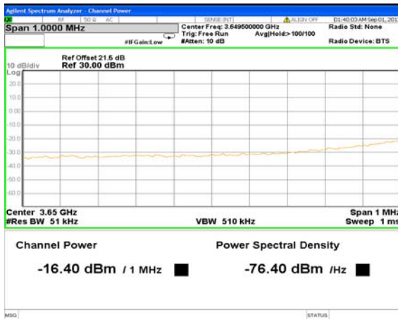
Plot # 78. Modulation BPSK. Output 20.8 dBm
