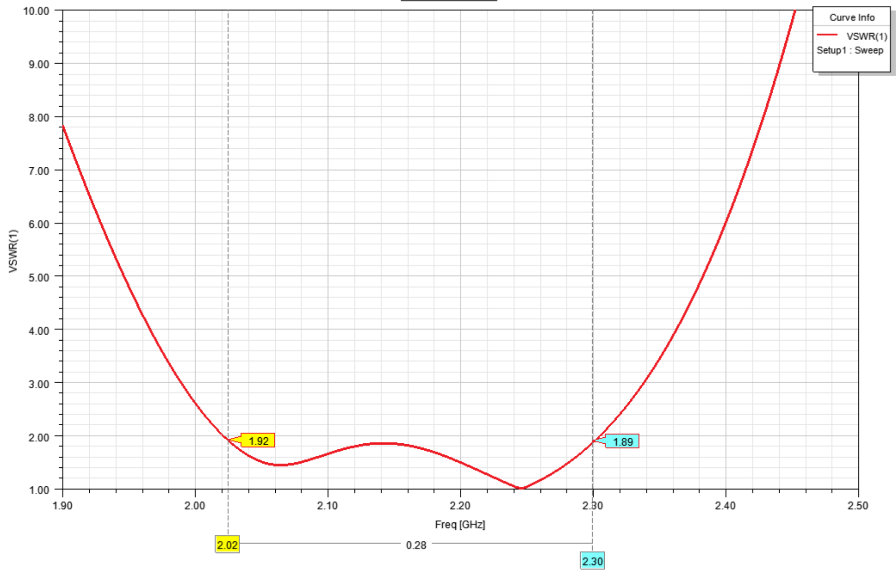
VSWR Plot 1
