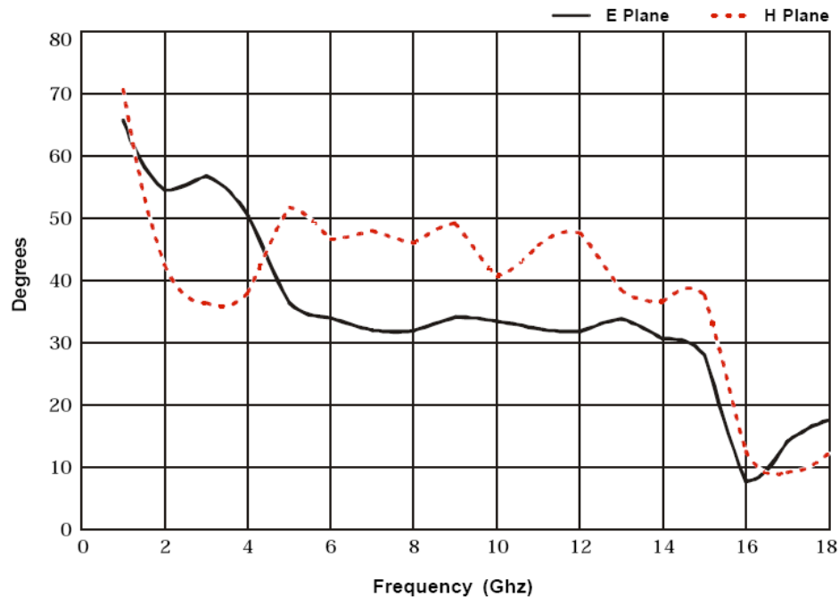
Model 3115 Half Power Beamwidth
