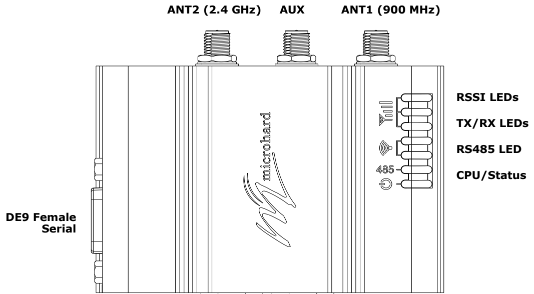
Figure 3-1: pDDL900/1800-ENC Top View
