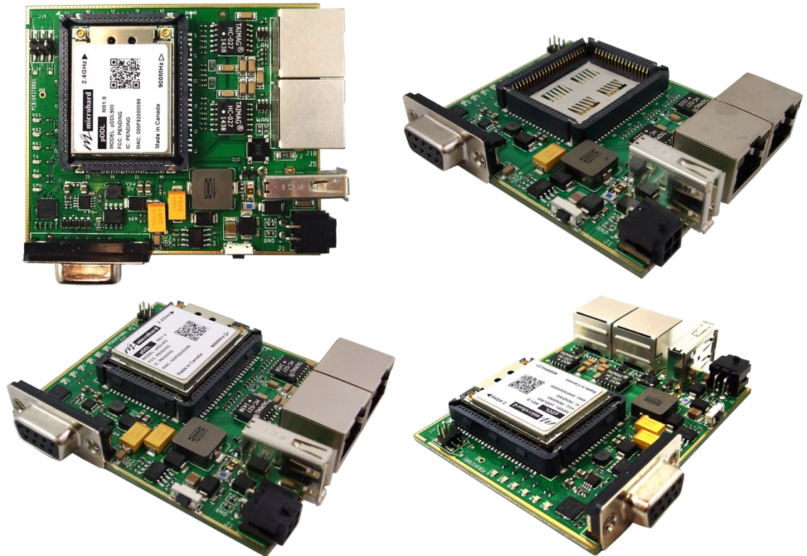
Image 3-4: pDDL900/1800 Development Board
