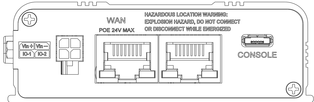
Figure 3-2: pDDL900/1800-ENC Back View
