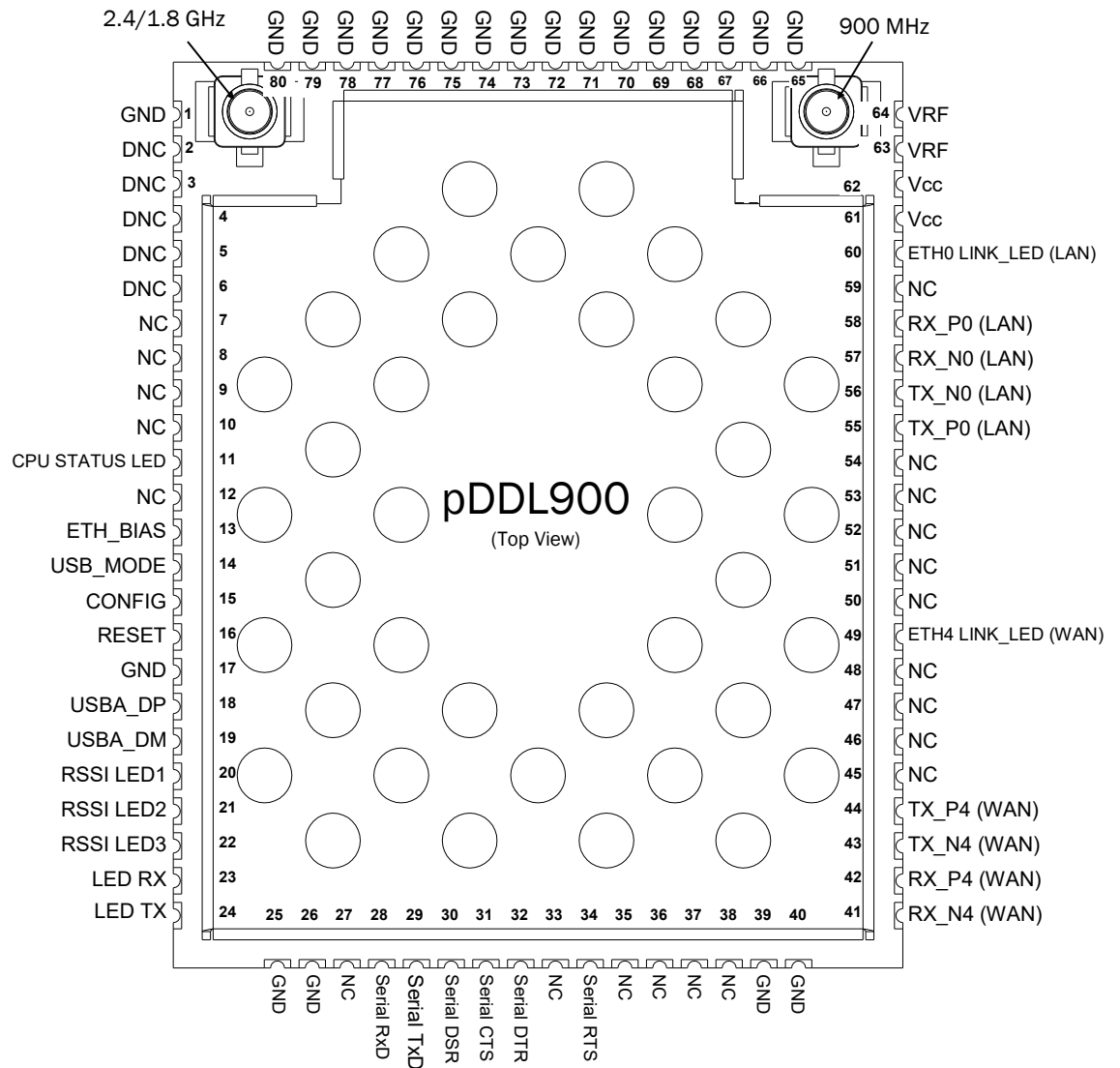
Drawing 3-5: pDDL900/1800 80-pin OEM Connection Info
