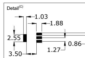
Drawing 3-3: pDDL900/1800 Recommended Solder Paste
