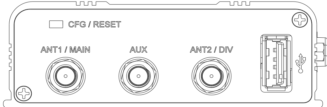
Figure 3-3: pDDL900/1800-ENC End View
