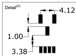
Drawing 3-3: pDDL900/1800 Recommended Solder Paste
