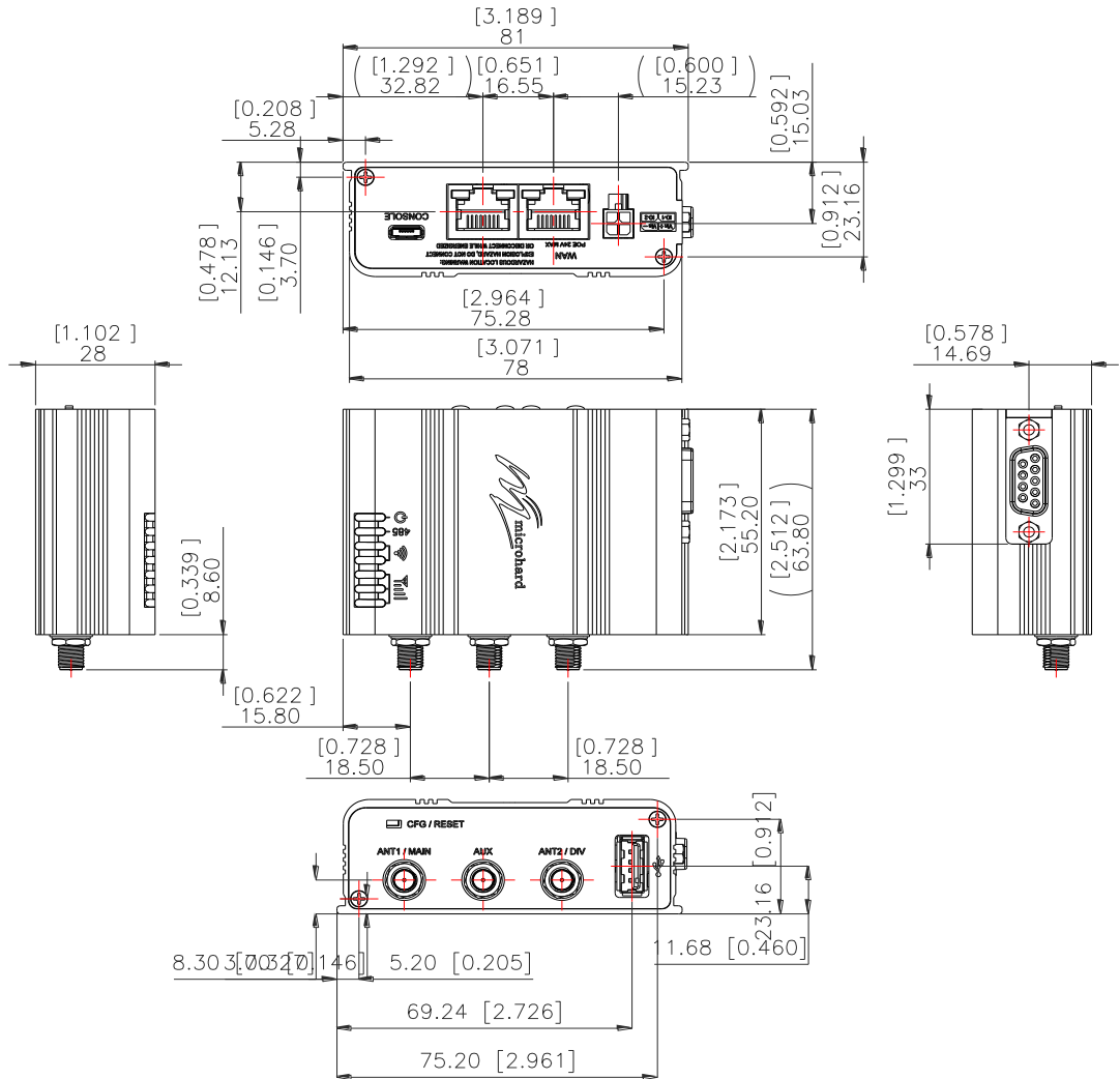
Drawing 3-7: pDDL900/1800-ENC Mechanical
