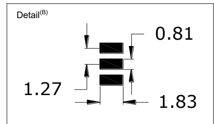
Drawing 3-2: pDDL900/1800 Recommended Solder Mask
