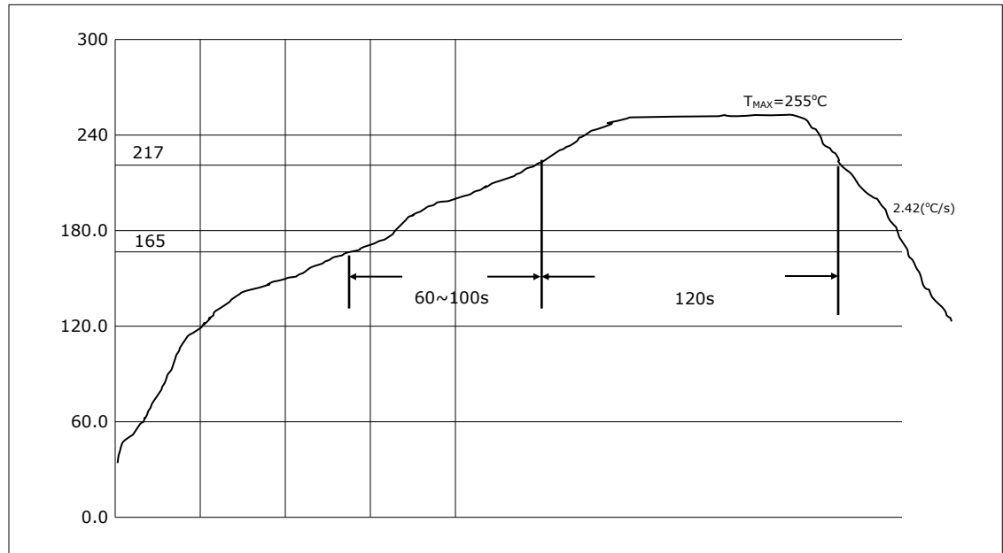
Drawing 3-4: pDDL900/1800 Reflow Profile
