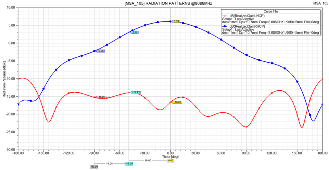
Figure 3. X-band TTnC Antenna Radiation Pattern
