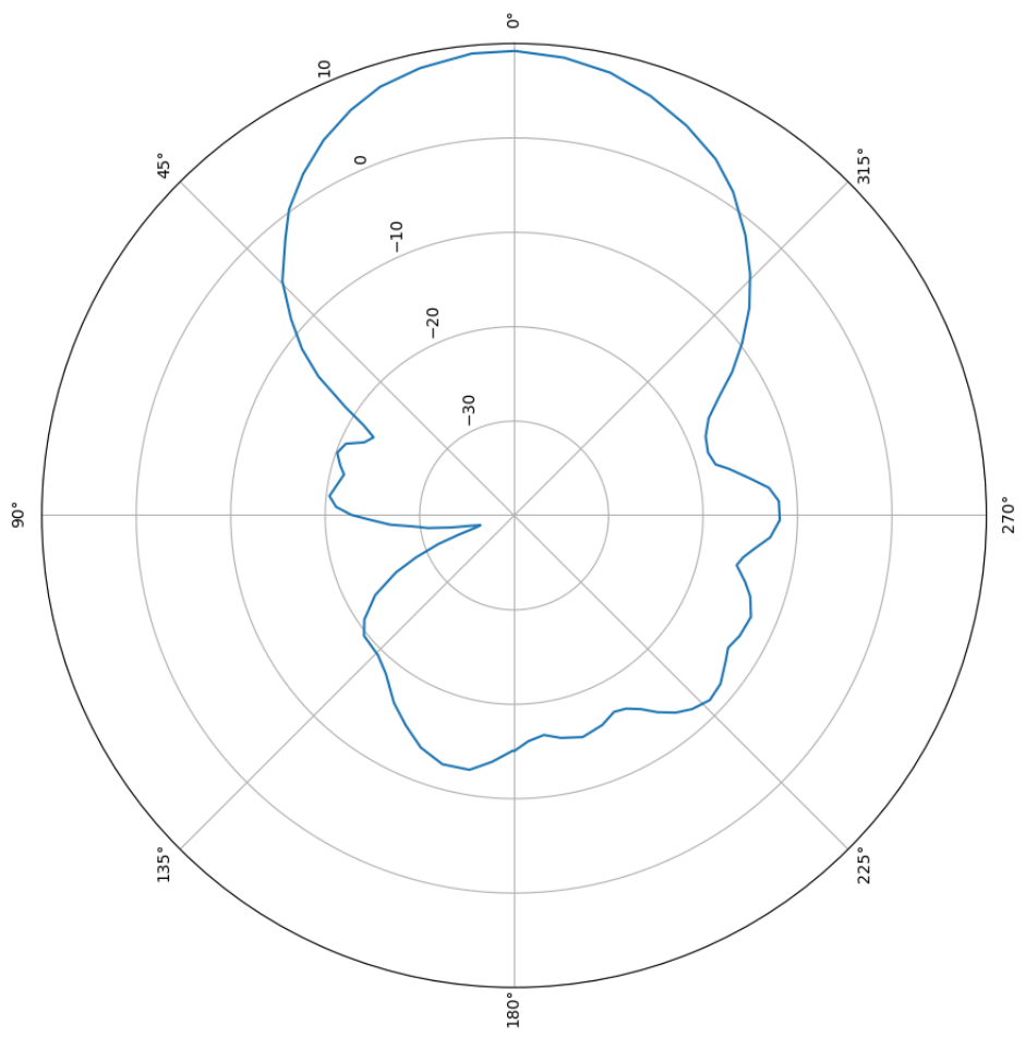
Gain (dB) @ 1525 MHz \phi = 0^\circ
