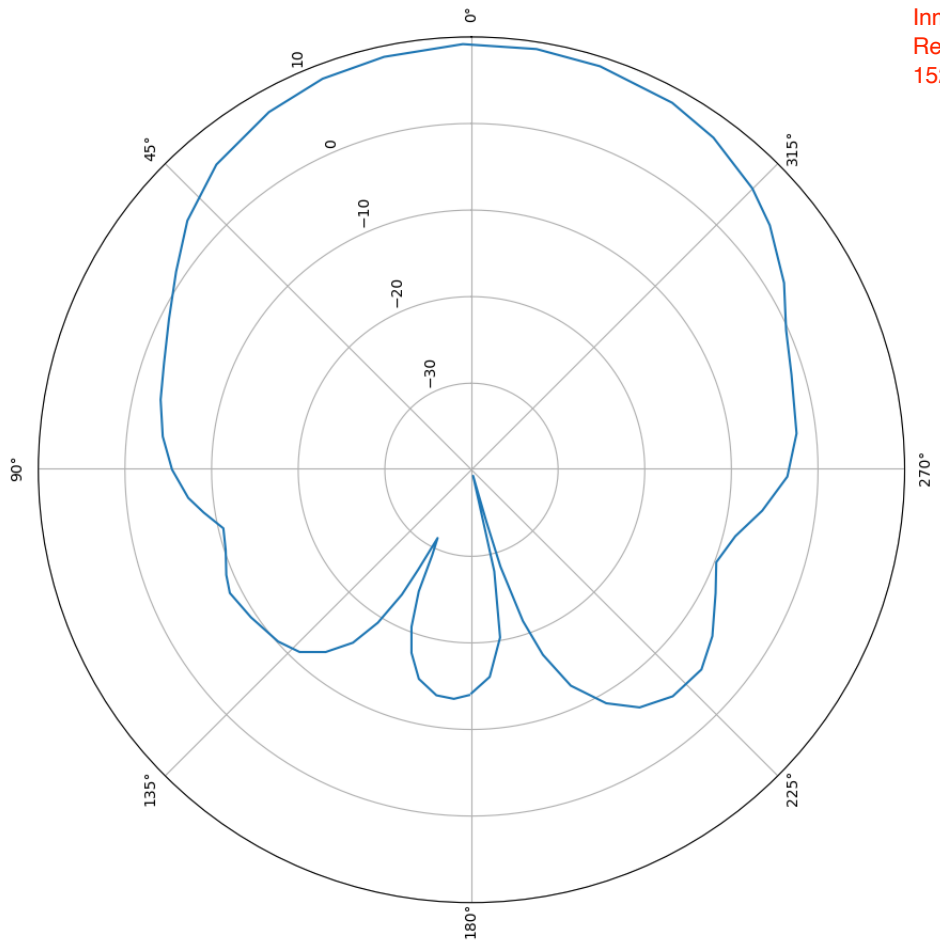
Gain (dB) @ 1525 MHz \phi = 90^\circ
