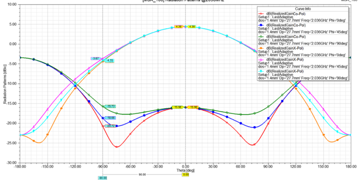
[MSA_106] Radiation Patterns @2036MHz
