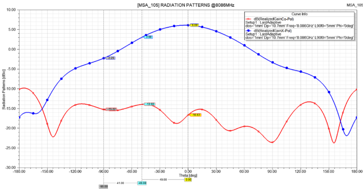
Capella TT&C Downlink Gain Pattern
