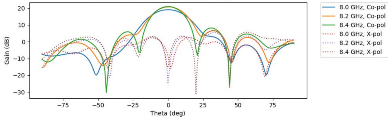
X-Band Payload Downlink Antenna Gain, \Phi=0
