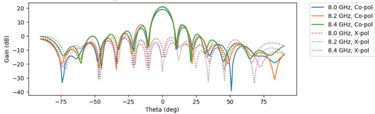
X-Band Payload Downlink Antenna Gain, \Phi=90
