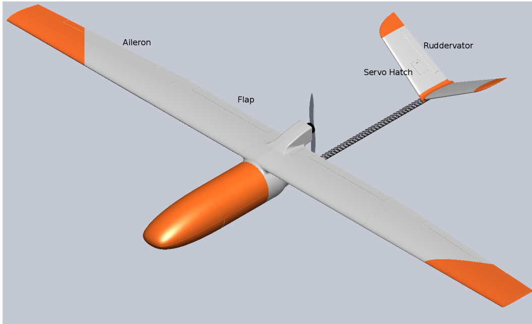
Figure – S2 Surface and Servo Location
