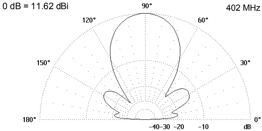
Figure 4: Earth Station UHF Transmit/Receive Antenna for Fairfax, VA and Las Vegas, NV.
