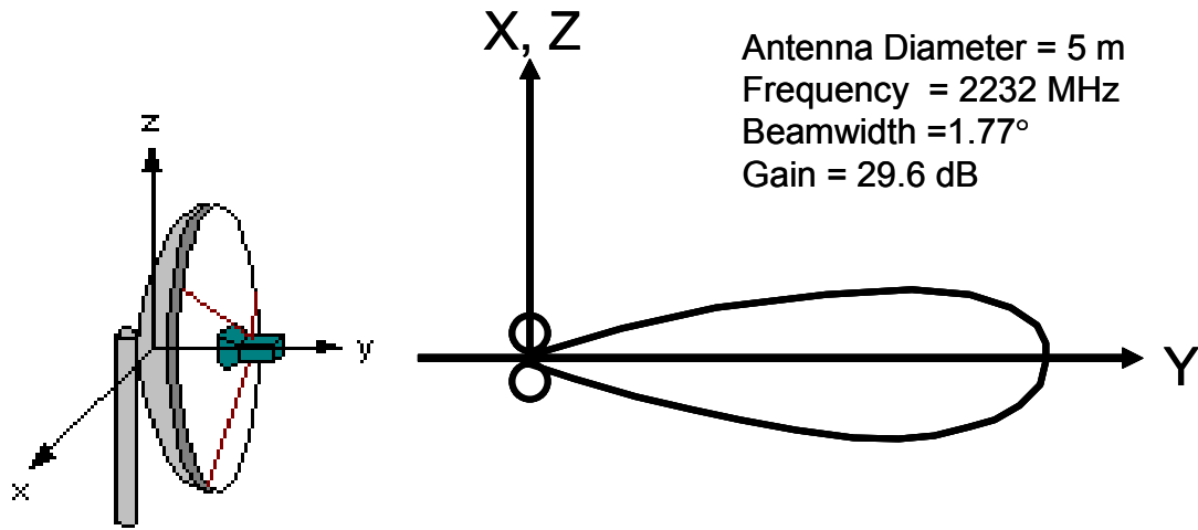
Figure 2: Earth Station S-Band Transmit/Receive Antenna for Fairfax, VA and Las Vegas, NV.
