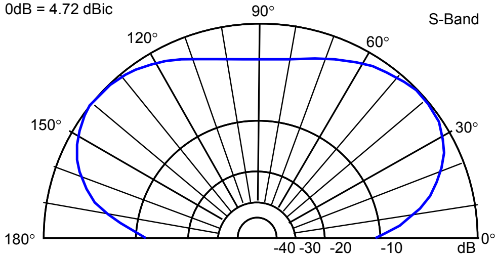
Figure 1: Space Station S-Band Transmit/Receive
