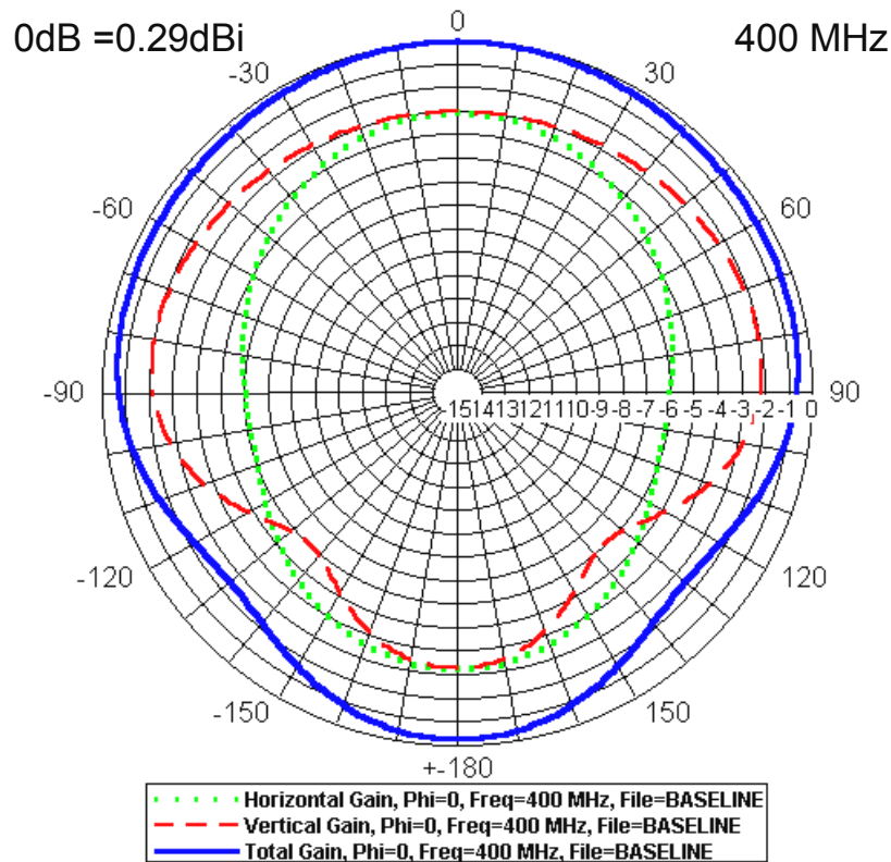
Figure 3: Space Station UHF Transmit/Receive Antenna
