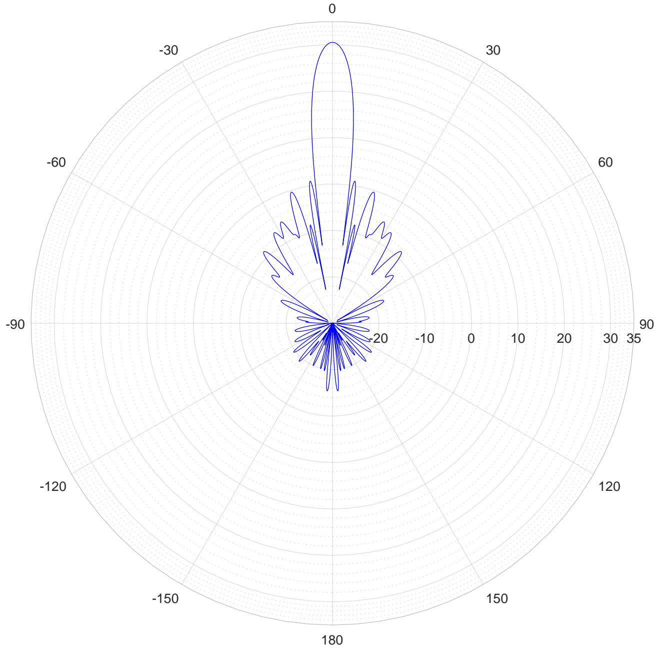
RHCP Directivity (dB), 2055 MHz, Peak Dir = 30.5 dB, HPBW = 5.5 deg 6 ft. dish, LHCP feed, 12 dB gaussian taper, 6" dia. feed blockage
