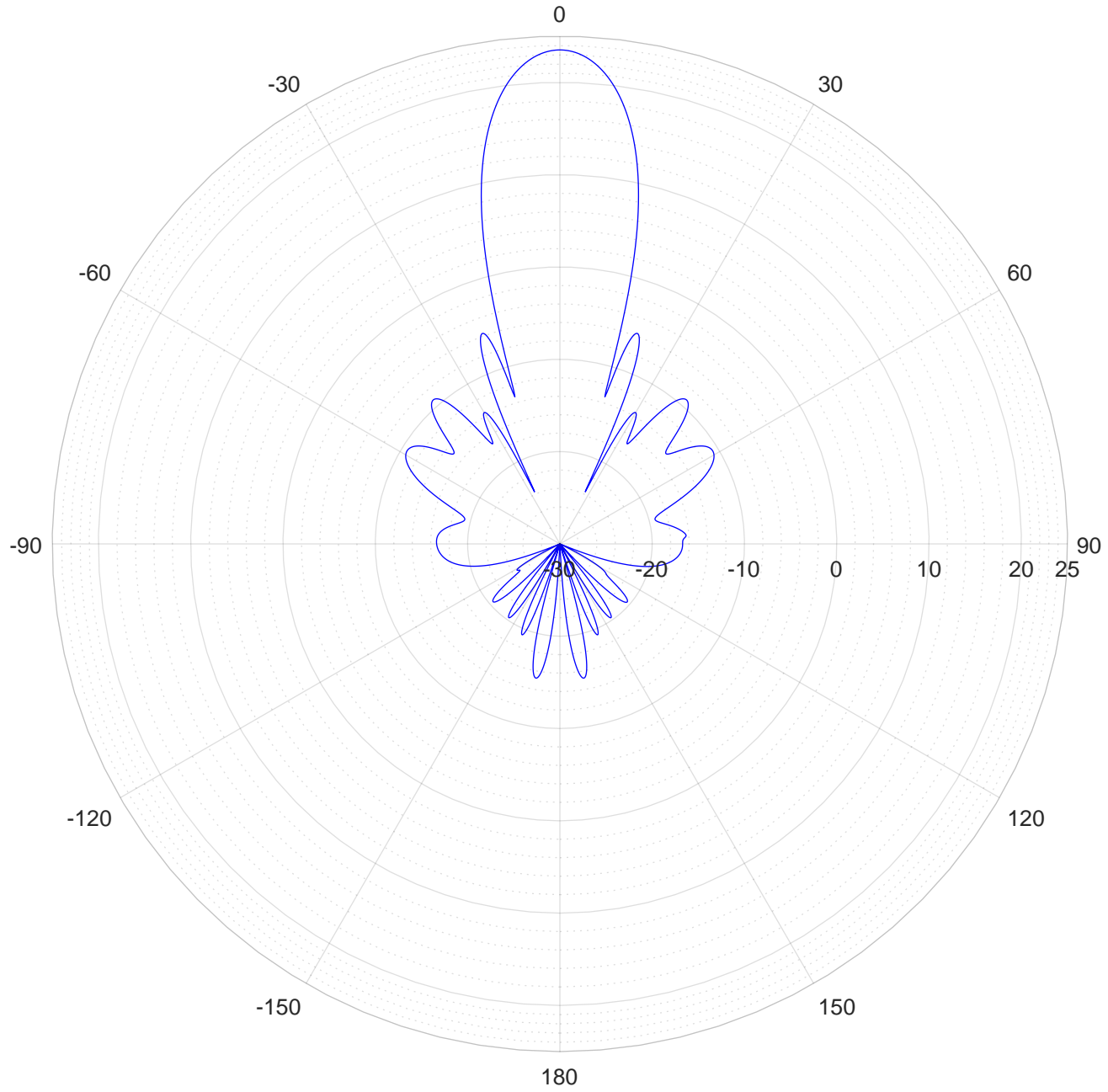
RHCP Directivity (dB), 915 MHz, Peak Dir = 23.5 dB, HPBW = 12 deg 6 ft. dish,LHCP feed, 12 dB gaussian taper, 6" dia. feed blockage
