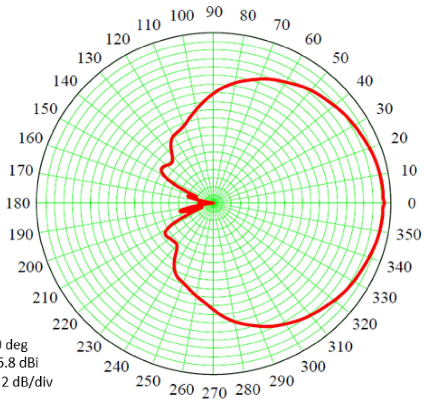
2250 MHz Representative Antenna Pattern
