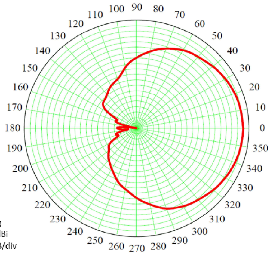
2080 MHz Representative Antenna Pattern
