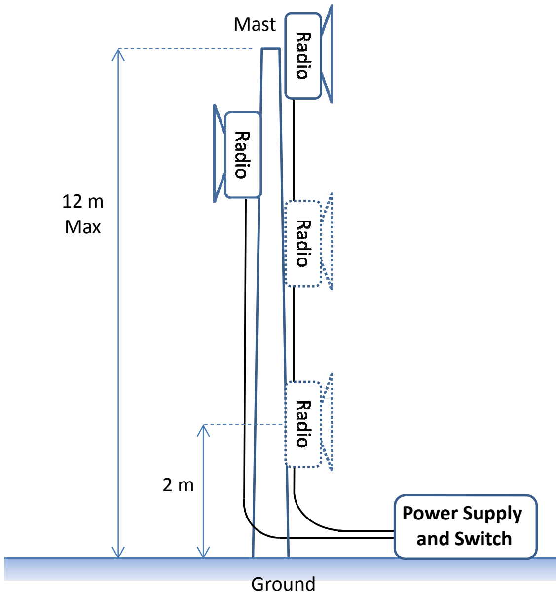
Figure 1 - Possible Radio Deployments on Mast
