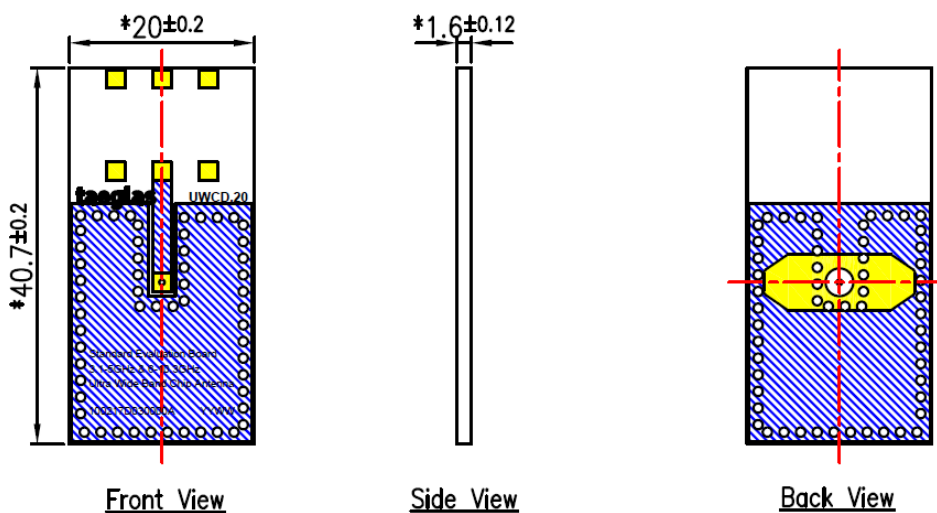
Figure 1 Evaluation Board
