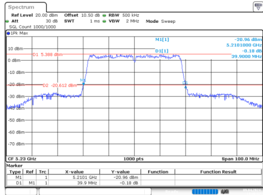
n40_5230MHz_Chain 0 39.900 MHz
