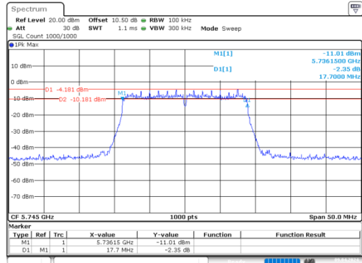
n20_5745MHz_Chain 0
