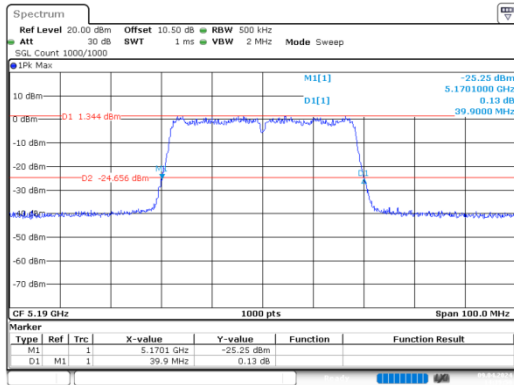
n40_5190MHz_Chain 0 39.900 MHz
