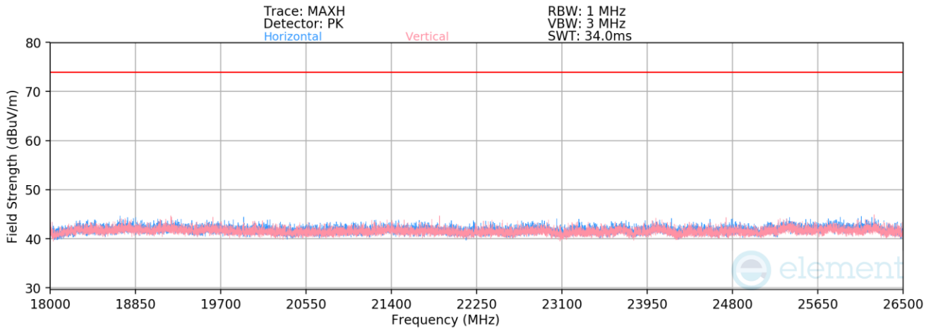
Plot 7-30. Radiated Spurious Emissions Above 18GHz (BT GFSK – Ch. 0)
