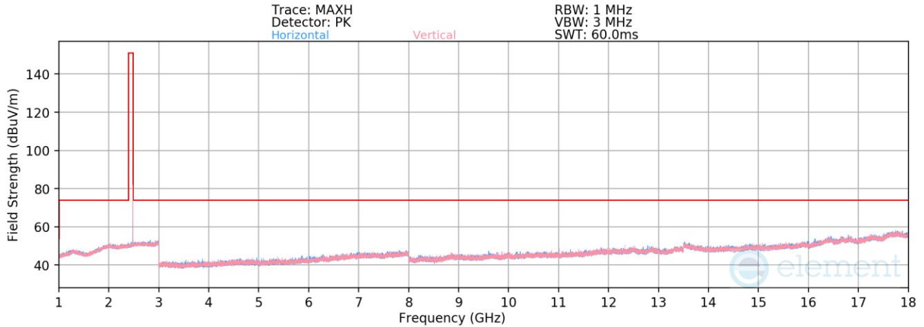
Plot 7-32. Radiated Spurious Emissions 1-18GHz (BT GFSK – Ch. 78)
