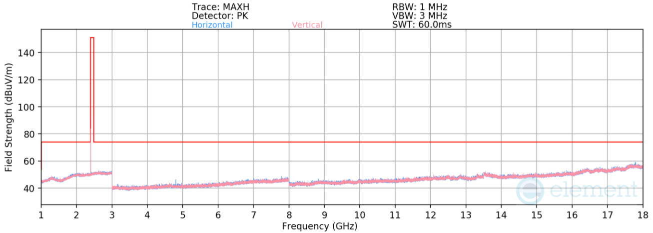
Plot 7-29. Radiated Spurious Emissions 1-18GHz (BT GFSK – Ch. 0)
