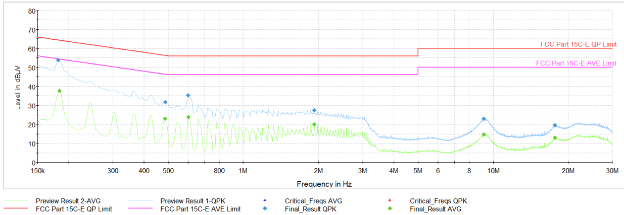
Plot 7-38. AC Line-Conducted Test Plot (L1, GFSK – Ch.0, with charging case and AC/DC Adapter)
