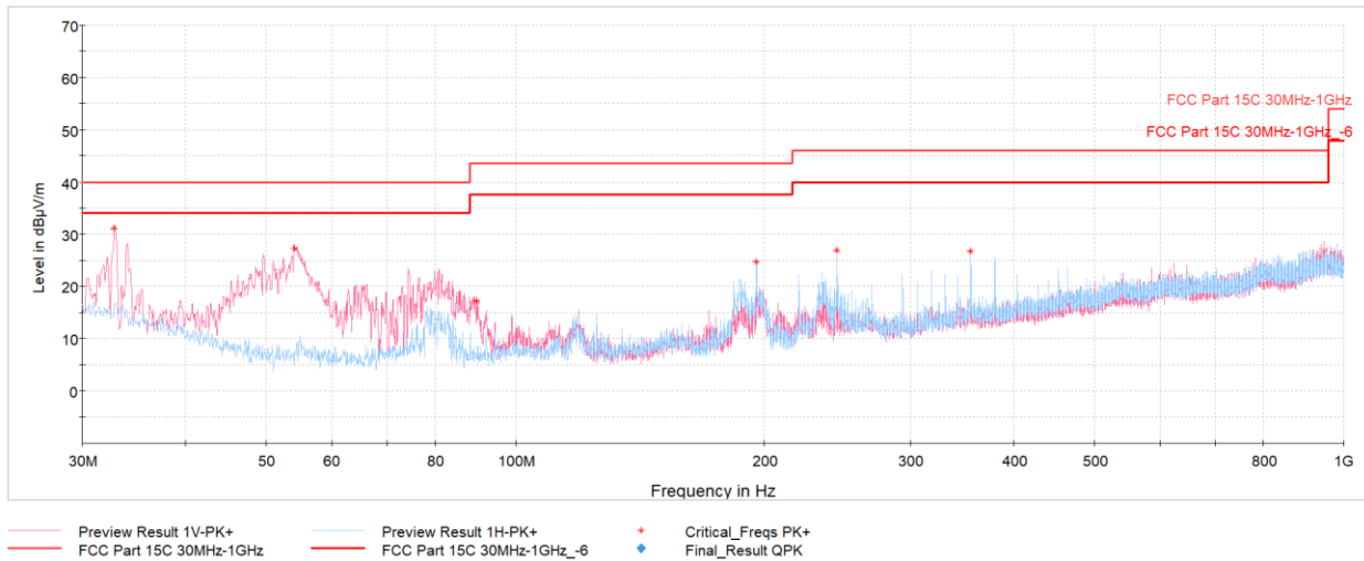
Plot 7-37. Radiated Spurious Emissions Below 1GHz (GFSK – Ch.0, with charging case and AC/DC Adapter)
