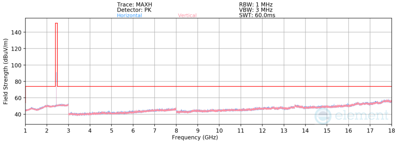
Plot 7-31. Radiated Spurious Emissions 1-18GHz (BT GFSK – Ch. 39)
