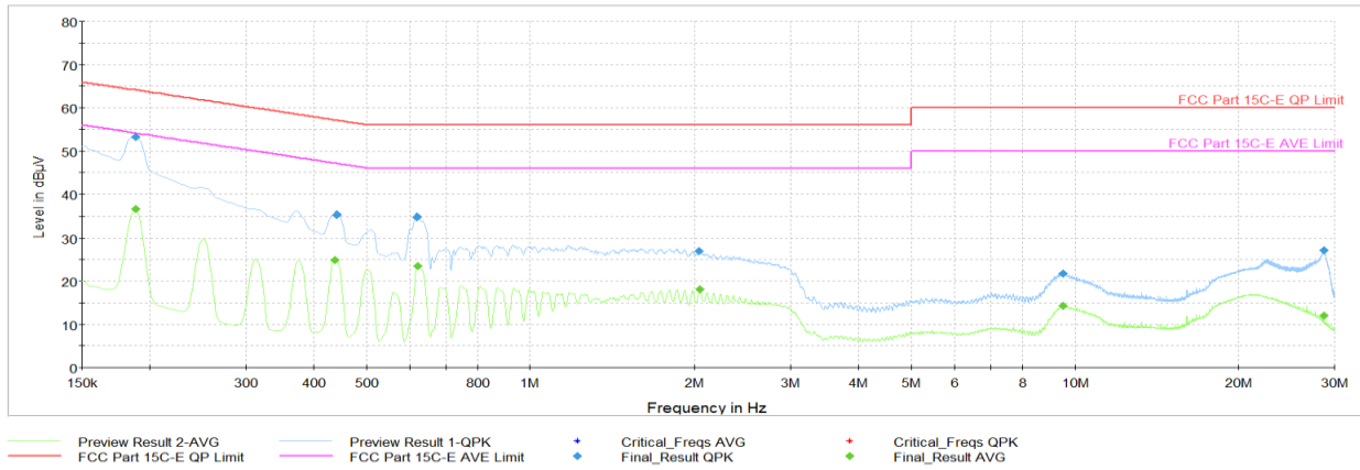
Plot 7-39. AC Line-Conducted Test Plot (N, GFSK – Ch.0, with charging case and AC/DC Adapter)
