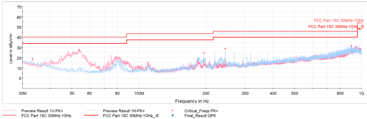
Plot 7-37. Radiated Spurious Emissions Below 1GHz (GFSK – Ch.78, with charging case and AC/DC Adapter)
