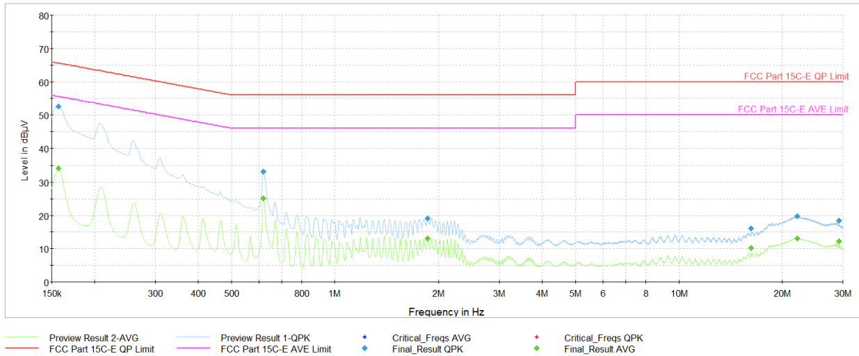
Plot 7-38. AC Line-Conducted Test Plot (L1, GFSK – Ch.78, with charging case and AC/DC Adapter)
