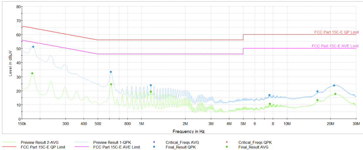
Plot 7-39. AC Line-Conducted Test Plot (N, GFSK – Ch.78, with charging case and AC/DC Adapter)
