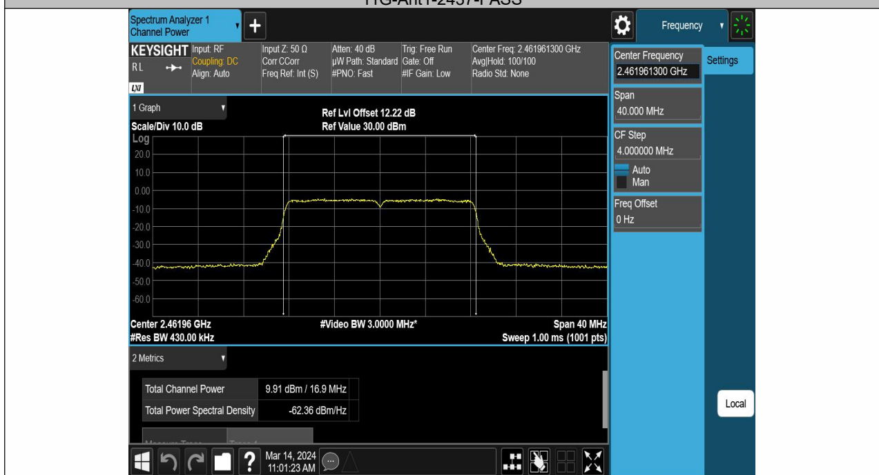
11G-Ant1-2462-PASS
