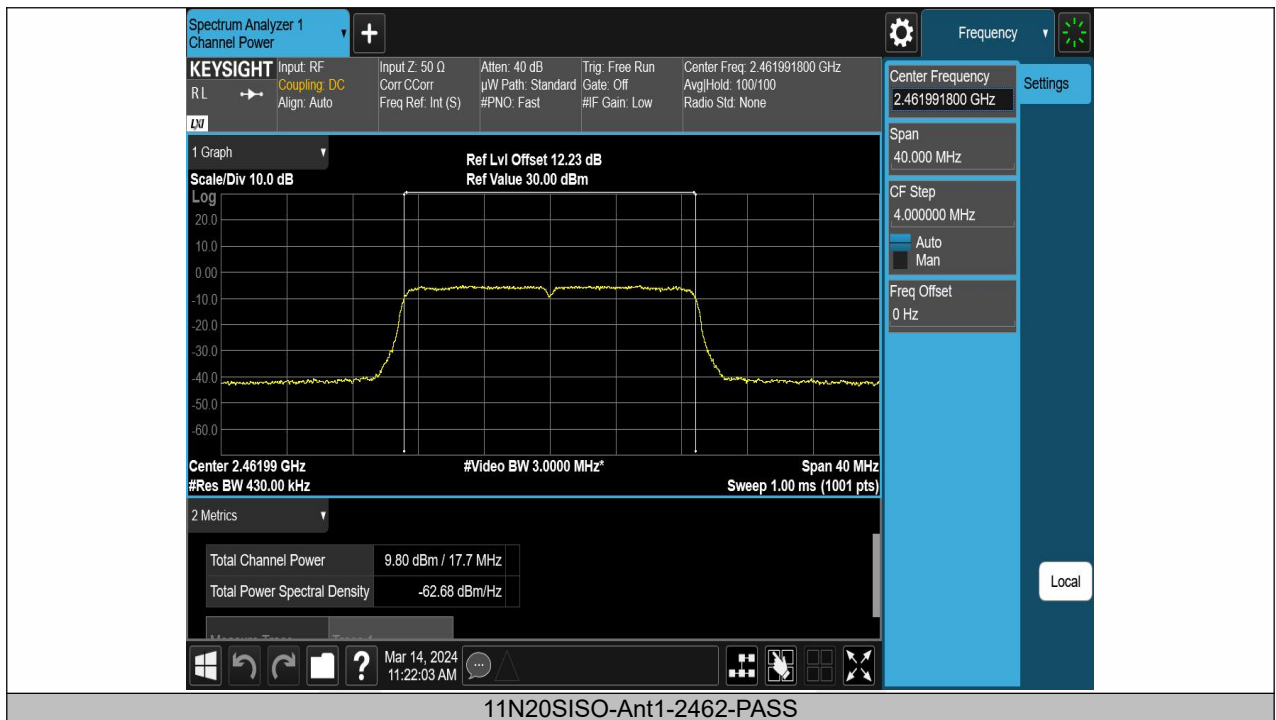
11N20SISO-Ant1-2462-PASS
