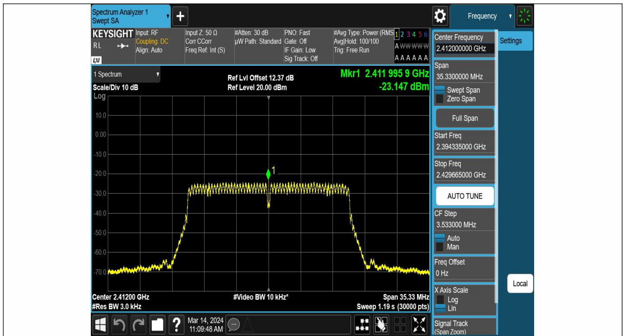
11N20SISO-Ant1-2412-PASS
