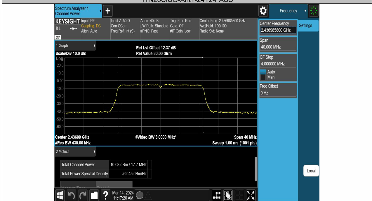
11N20SISO-Ant1-2437-PASS
