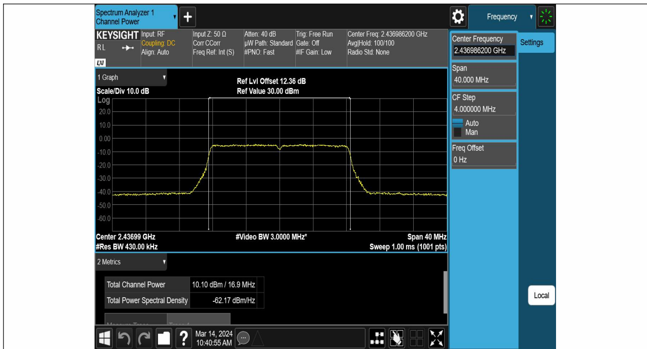
11G-Ant1-2437-PASS
