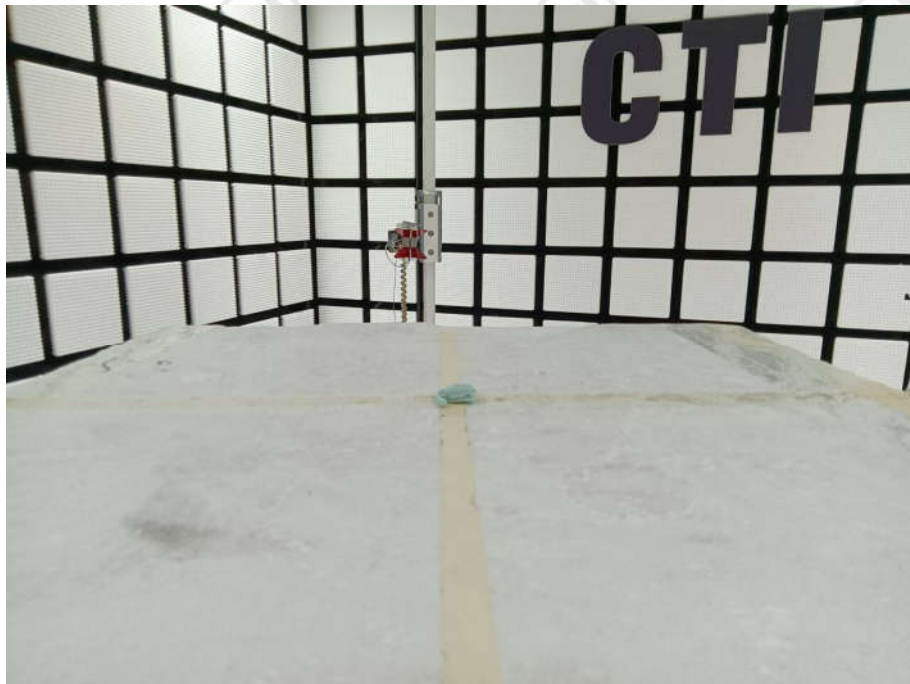
Radiated spurious emission Test Setup-4(Above 1GHz)(right ear)
