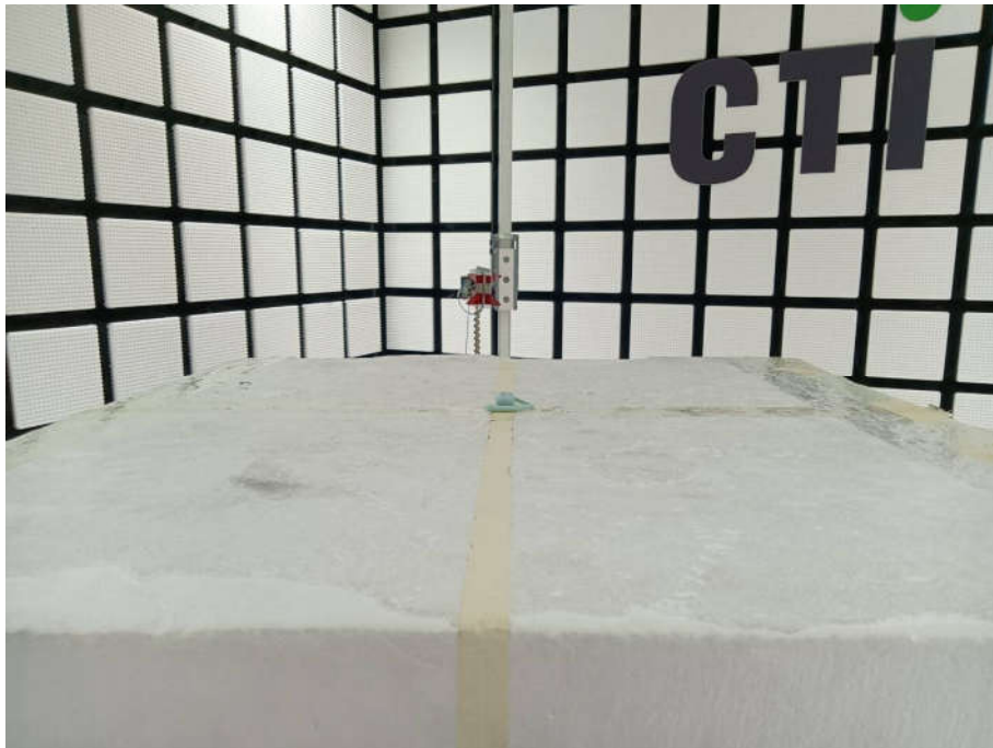
Radiated spurious emission Test Setup-2(Above 1GHz)(left ear)
