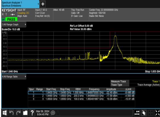
N2(20M)_DFT-s- OFDM_QPSK_Edge_1RB_Left_Low_CH
