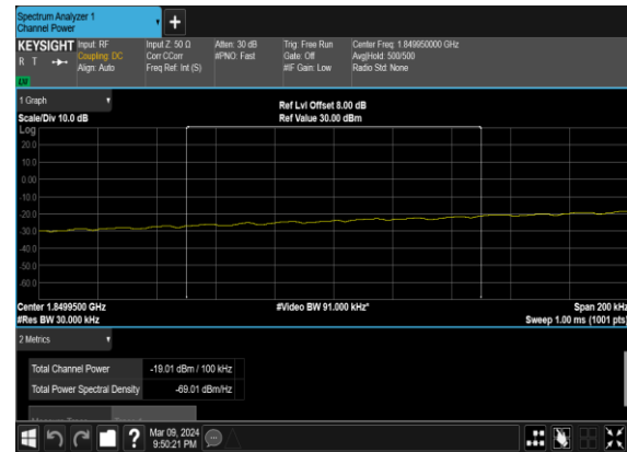
N2(10M)_DFT-s-OFDM_BPSK_Edge_1RB_Left_Low_CH_CHP_PA SS
