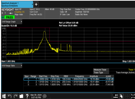
N2(20M)_DFT-s- OFDM_QPSK_Edge_1RB_Right_High_CH
