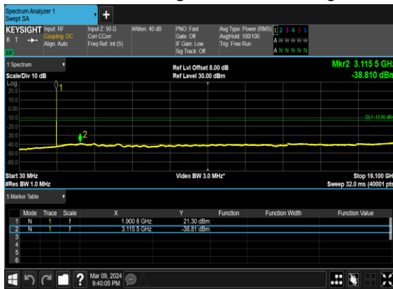
N2(10M)_DFT-s-OFDM_BPSK_Edge_1RB_Left_High_CH
