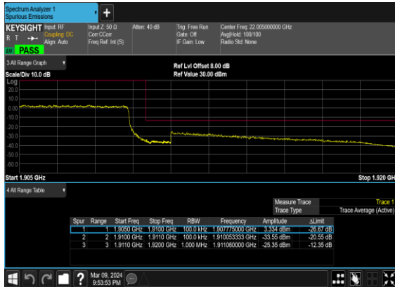
N2(10M)_DFT-s-OFDM_QPSK_Outer_Full_High_CH
