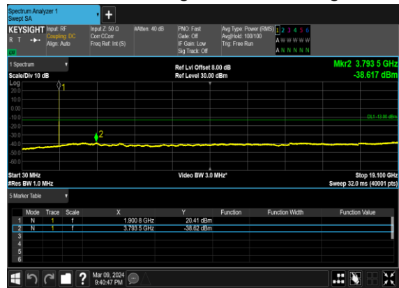
N2(10M)_DFT-s-OFDM_QPSK_Edge_1RB_Left_High_CH
