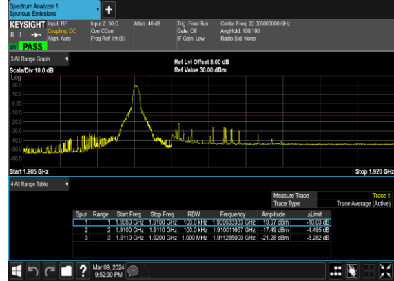
N2(10M)_DFT-s-OFDM_BPSK_Edge_1RB_Right_High_CH
