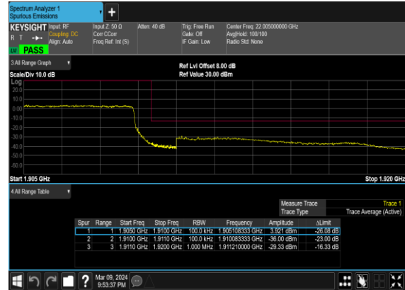
N2(10M)_DFT-s-OFDM_BPSK_Outer_Full_High_CH
