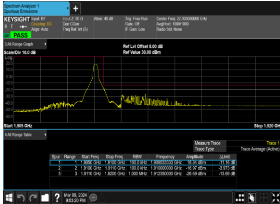
N2(10M)_DFT-s-OFDM_QPSK_Edge_1RB_Right_High_CH
