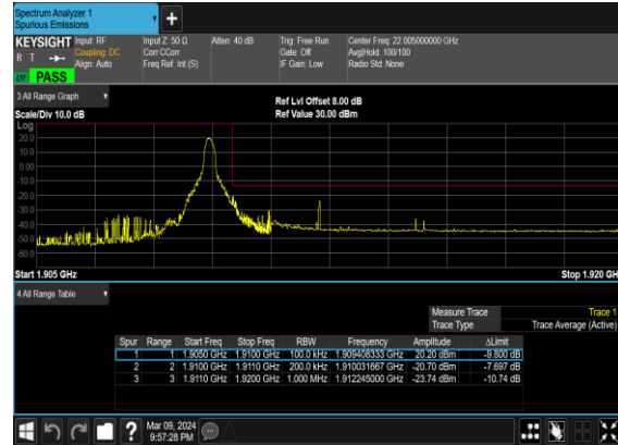
N2(20M)_DFT-s- OFDM_BPSK_Edge_1RB_Right_High_CH
