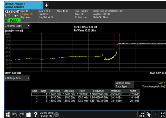
N2(10M)_DFT-s-OFDM_BPSK_Outer_Full_Low_CH
