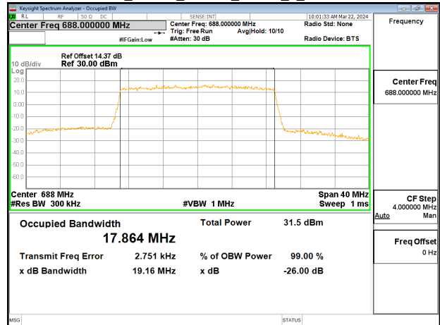
Band71_20MHz_16QAM_RB100_0_CH133372
