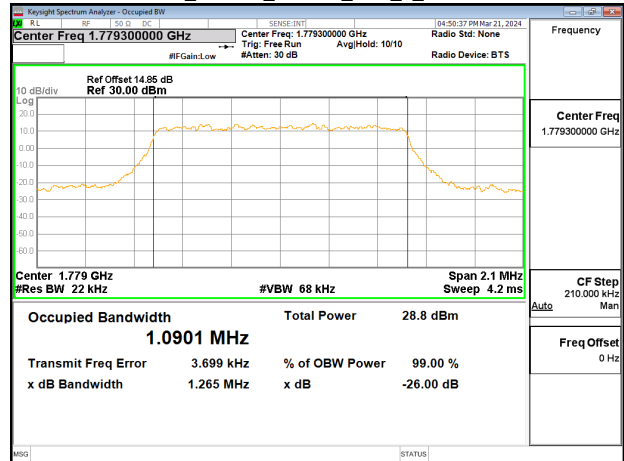
Band66 1.4MHz_16QAM_RB6_0_CH132665
