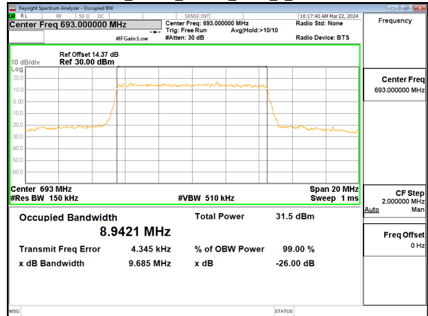
Band71_10MHz_16QAM_RB50_0_CH133422
