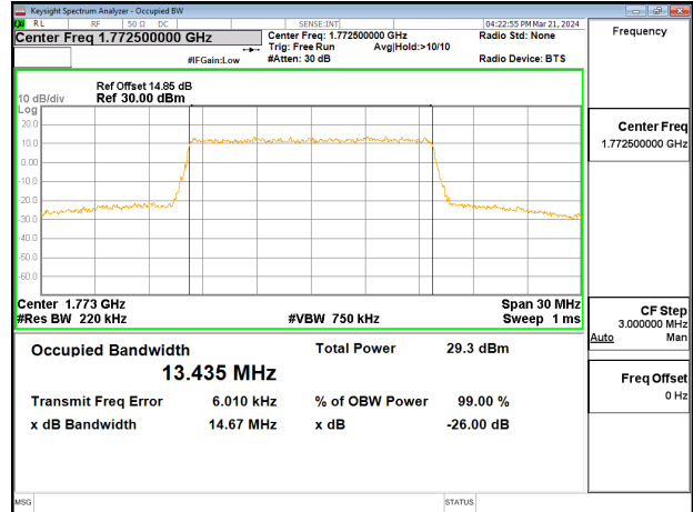
Band66_15MHz_16QAM_RB75_0_CH132597
