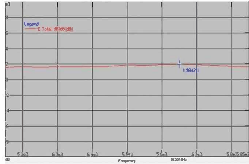
Maximum Peak Gain at 5650 MHz : 1.96 dBi
