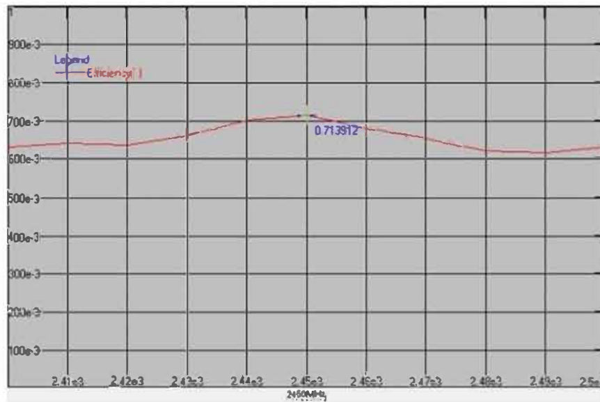
Maximum Efficiency at 2450 MHz 71.39%
